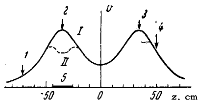
FIG. 2. Effective potential of magnetic trap on the axis: U = H_z + e\varphi ; I – without electric field ( \varphi = 0 ), II – with electric field of the ring; 1 – location of gun, 2 – first magnetic mirror, 3 – second magnetic mirror, 4 – location of collector, 5 – location of ring.
