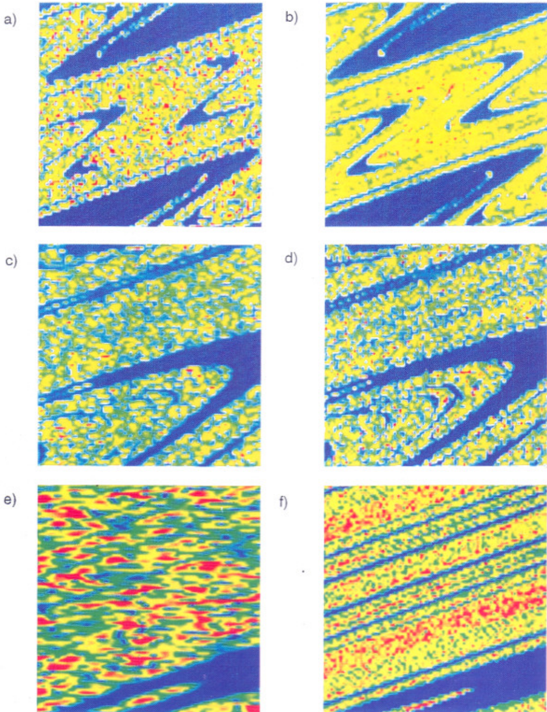
Fig. 1. Left column: Husimi function of the quantum fractal eigenstate for N = 59049 and \Gamma = 0.1080 \approx \gamma_c . Right column: classical strange repeller obtained, from initially homogeneously distributed orbits, after 100 iterations of map (2). The color varies proportionally to the density: from blue for zero density to bright red for maximal density (the color scale is the same for classical and quantum cases on each magnification level). The size of the phase region (\theta, n) is: 0 \leq \theta \leq 2\pi , -N/2 \leq n \leq N/2 for (a) and (b); 0 \leq \theta \leq 2\pi/3 , -N/6 \leq n \leq N/6 for (c) and (d); 0 \leq \theta \leq 2\pi/9 , -N/18 \leq n \leq N/18 for (e) and (f).
