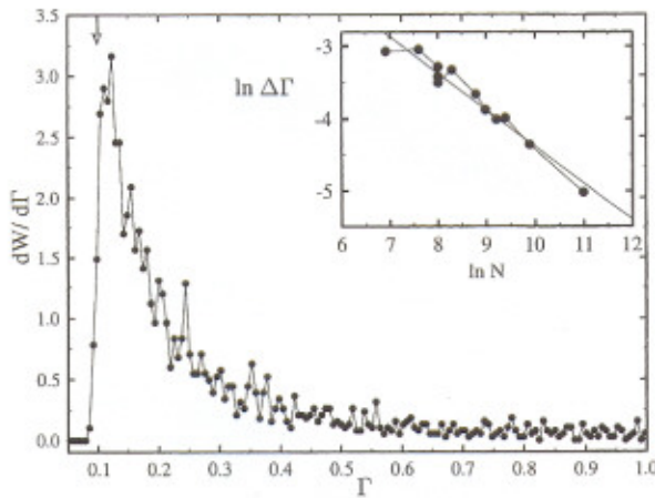
Fig. 2. Distribution dW/d\Gamma as a function of \Gamma for N = 12001 . The arrow marks the value of \gamma_c . The inset shows \Delta\Gamma = \gamma_c - \Gamma_{\min} vs. N in log-log scale. The straight line shows the dependence given by (3). To guide the eye, the numerical data (points) are connected by lines.
