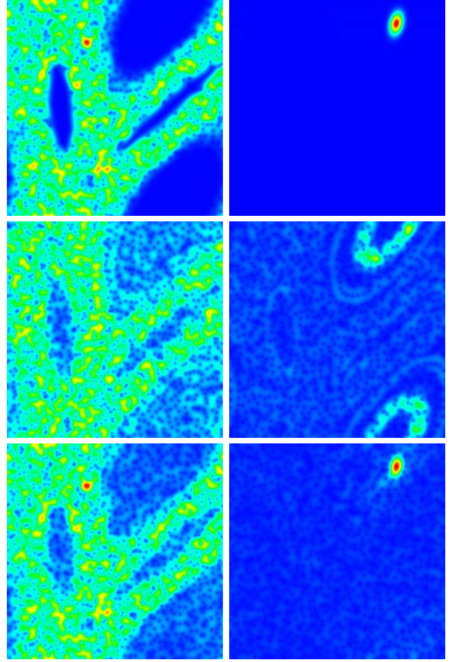
Fig. 2. Quantum Poincaré sections with Husimi-functions at t = 3000 in scaled momentum and position variables \tilde{y} = p[l/(2\pi\hbar)] \in [0, 2\pi] and \tilde{x} = x[2\pi/l] \in [0, 2\pi] : the parameters are K = 1.7 and n_q = 10 . The initially prepared coherent states are centered around (\pi/4, 0) (left panel) and (5.35, 0) (right panel). First row: ideal dynamics; second row: static imperfections with \epsilon = 5 \times 10^{-6} ; third row: PAREC-method applied after each sequence of n_{\text{gef}} = 20 universal quantum gates of reference [12]. The probability density is coded in colors (red/maximum, blue/zero).
