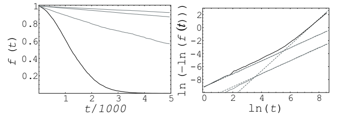
Fig. 3. Dependence of the fidelity f(t) on the number of iterations: parameters as in the left panel of Figure 2; left: static imperfections without error correction, PAREC after each map iteration, after each n_{\text{gef}} = 50 , and after each n_{\text{gef}} = 20 quantum gates (from bottom up); right: static imperfections without error correction, with PAREC after each map iteration and after each sequence of n_{\text{gef}} = 20 quantum gates (full curves), best fits for linear- and quadratic-in-time decays (dashed curves).
