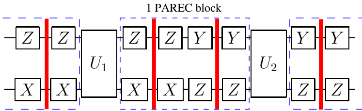
Fig. 3. (Color online) Schematic representation of the PAREC method. The vertical thick (red) lines indicate the place where the static coupling propagator U_{\text{stat}} is applied. In order to preserve \text{tr}[\delta H^2] we take \epsilon/2 for each propagator. The dashed lines enclose a PAREC block. Repetition of PAREC between two gates means applying repeatedly one PAREC block after another.
