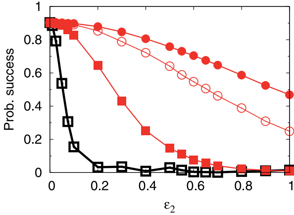
Fig. 4. (Color online) Success probability of IQPEA which determines the phase with a precision of up to 10 bits, in the presence of static imperfections, as a function of the imperfection strength \epsilon_2 . The curves show the influence of PAREC and how probability is enhanced with the increase of the number of times PAREC is applied: (□) No PAREC; (■) 1 time; (○) 5 times; (●) 10 times. No random imperfections are present ( \epsilon_1 = 0 ). Averaging is done over 2000 randomly chosen phases.
