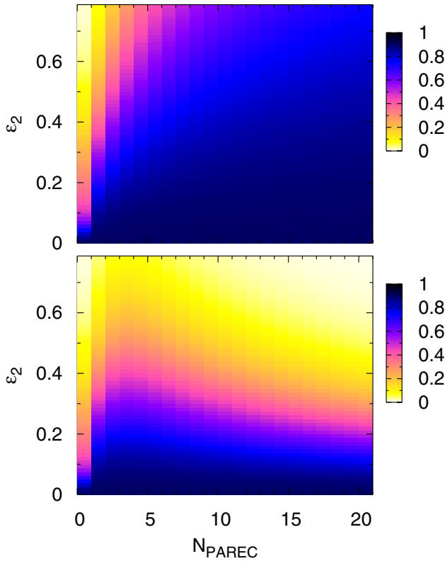
Fig. 5. (Color online) Success probability (shown by color) of the IQPEA which determines the phase with a precision of up to 2^{-10} as a function of the number of times N_{\text{PAREC}} PAREC is applied and of the static imperfections strength \epsilon_2 . Top: the case where only static imperfections are considered ( \epsilon_1 = 0 ). Bottom: both static and random imperfections are present (including in PAREC gates); here random errors in gates are also present, their strength is taken as \epsilon_1 = \epsilon_2/5 . Averaging is done over 2000 randomly chosen phases.
