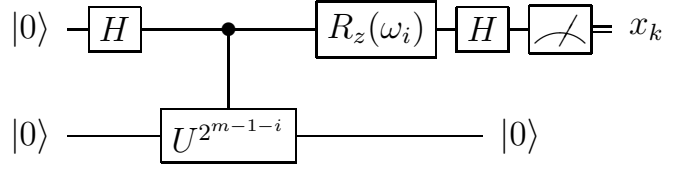
Fig. 1. Step i (where i = 0, \dots, m-1 ) of the IQPEA of [6]. Here R_Z is a rotation by an angle \omega_i around \hat{z} axis.
