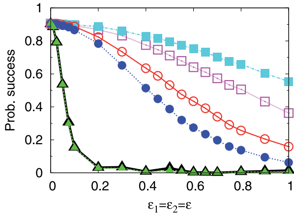
Fig. 2. (Color online) Success probability for the algorithm to determine the phase with a precision of up to 10 bits, as a function of the parameter \epsilon = \epsilon_1 = \epsilon_2 characterizing the error strength. Symbols mark: random phase errors in the Hadamard gates ( \square ), the R_z gate ( \blacksquare ), the controlled- U^{2^k} ( \circ ) and errors in all of the gates ( \bullet ). The case of static imperfections is shown by ( \triangle )/( \blacktriangle ) in absence/presence of random phase errors in the gates. Averaging is done over 2000 randomly chosen phases.
