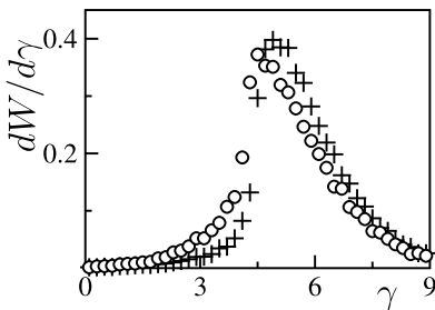
Fig. 4. Dependence of the density of states dW/d\gamma of \mathbf{G} on the relaxation rate \gamma = -2\ln|\lambda| for unweighted (pluses) and weighted (circles) links in the neuronal network.
