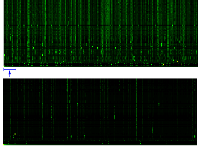
FIG. 6: (Color online) Coarse-grained probability distribution |\psi_i(j)|^2 for the eigenstates of the Google matrix for Linux Kernel version 2.6.32. The horizontal lines show the first 64 eigenvectors ordered vertically by |\lambda_i| from |\lambda| = 1 on bottom to |\lambda| \approx 0.4 on top (only one state is shown for degenerate eigenvalues, all states are normalized by \sum_j |\psi_i(j)|^2 = 1 , index j corresponds to the order given by the PageRank located at the bottom line). The top panel shows the coarse-grained complete network of 285509 sites with 307 cells, each containing 930 sites; the bottom panel shows the coarse-grained distribution for first 300 cells, each containing 62 sites (bar and arrow on the top panel mark the region of bottom panel). Probability is proportional to color with black for zero and yellow/white for maximum.
