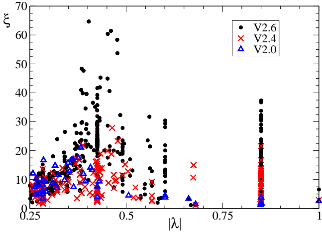
FIG. 5: (Color online) Localization properties of Google matrix eigenstates for Linux Kernel versions 2.0.40 2.4.37.6 and 2.6.32 with N = 14079, 85756, 285509 respectively. The participation ratio \xi of eigenstates is shown as a function of modulus of the corresponding eigenvalues |\lambda| ; the values of \langle \xi \rangle , averaged over all given interval of |\lambda| , are 9.5, 8.6, 17.3 respectively.
