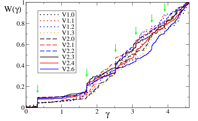
FIG. 2: (Color online) Dependence of the integrated density of states W on the relaxation rate \gamma = -2 \ln |\lambda| for the Google matrix of different versions of Linux Kernels from V1.0 with N = 14079 to 2.6.32 with N = 285509 as it is shown on the legend. The highly degenerate values of \gamma are marked by arrows at \gamma_m = -2 \ln(\alpha/m) for m = 1, 2, 3, 4, 5, 6 .
