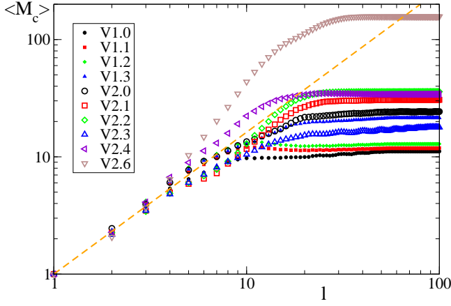
FIG. 4: (Color online) Cluster growing fractal dimension of the Linux Kernel networks. The average mass \langle M_c \rangle , with uniformly distributed seed, is shown for different Kernel versions as a function of the network distance l , in logarithmic scale. The dashed line represents the power law dependence corresponding to fractal dimension d = 1.21 , with \langle M_c \rangle \propto l^d .
