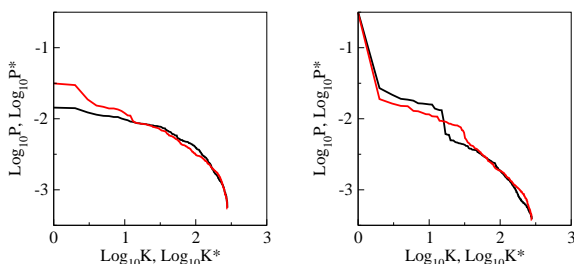
Fig. 3: (Colour on-line) Left panel : dependence of PageRank (CheiRank) probability P(K) ( P^*(K^*) ) on its index K ( K^* ) shown by black (red) curve. Right panel : dependence of ImpactRank probability P ( P^* ) on its index K ( K^* ), obtained via propagator of G ( G^* ) at \alpha = 0.85 and \gamma = 0.7 for the initial probability located on neuron RMGL (see text).
