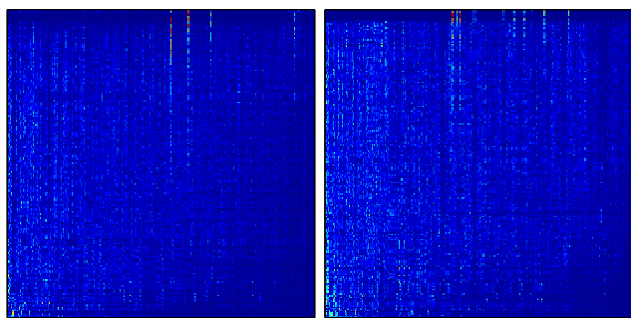
Fig. 6: (Colour on-line) Dependence of amplitude of eigenstates |\psi_i(K)| of G and |\psi_i^*(K^*)| of G^* on PageRank index K (left panel) and CheiRank index K^* (right panel); here x -axis shows values of K and K^* , while y -axis shows index i of eigenstates being ordered in a decreasing order of |\lambda_i| (see text). The whole index range 1 \leq K, K^* \leq 279 is shown with PageRank (CheiRank) vector being at the bottom line of each panel. The color is proportional to |\psi_i(j)| changing from minimum blue value to maximum value in red.
