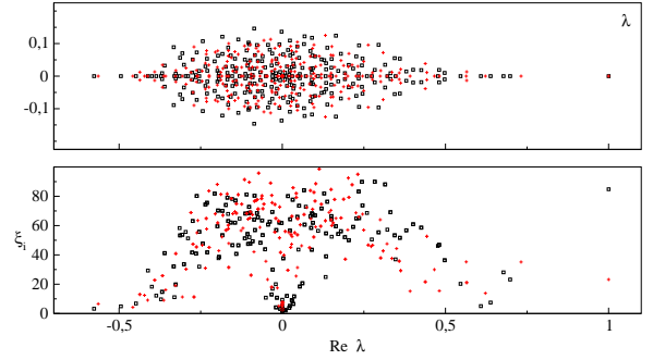
Fig. 2: (Colour on-line) Top panel: spectrum of eigenvalues \lambda for the Google matrices G and G^* at \alpha = 0.85 (black and red symbols). Bottom panel: IPR \xi of eigenvectors as a function of corresponding Re \lambda (same colors).
