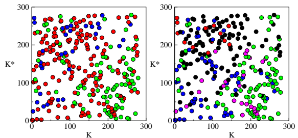
Fig. 4: (Colour on-line) PageRank - CheiRank plane ( K, K^* ) showing distribution of neurons according to their ranking. Left panel : soma region coloration - head (red), middle (green), tail (blue). Right panel : neuron type coloration - sensory (red), motor (green), interneuron (blue), polymodal (purple) and unknown (black). The classifications and colors are given according to WormAtlas [7].
