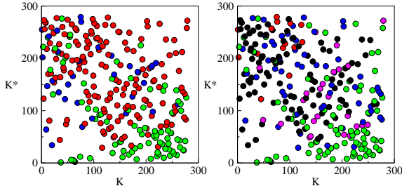
Fig. 5: (Colour on-line) Distribution of neurons in the plane (K, K^*) of equal opportunity ranks (see text); colors are the same as in Fig. 4.
