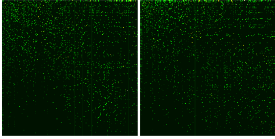
Fig. 1: (Colour on-line) Google matrix G (left) and G^* (right) for the neural network of C.elegans for N = 279 connected neurons. Matrix elements G_{KK'} are shown in the basis of PageRank index K (and K' ) and elements G_{K^*,K^{*}'} are shown in the basis of CheiRank index K^* (and K^{*}' ) at \alpha = 0.85 . Here, x and y axes show 1 \leq K, K' \leq N and 1 \leq K^*, K^{*}' \leq N ; the elements G_{11}, G_{11}^* are placed at the top left corner; color is proportional to the square root of matrix elements which are changing from black at minimum value (1 - \alpha)/N to light yellow at maximum.
