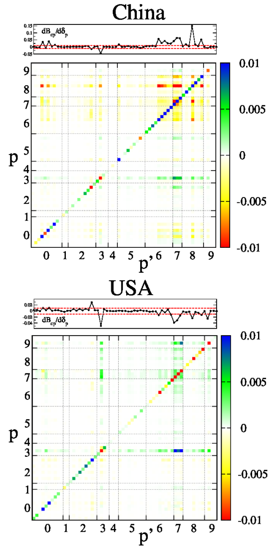
Fig. 24. China (top) and USA (bottom) examples of derivative dB_{cp}/d\delta_p of partial probability balance B_{cp} of product p over price \delta_p of product p' for year 2008. Diagonal terms, given by dB_{cp}/d\delta_p vs. p = p' , are shown on the top panels of each example. Products p' and p are shown in x -axis and y -axis respectively (indexed as in Table 1), while dB_{cp}/d\delta_p is represented by colors with a threshold value given by -0.01 and 0.01 for negative and positive values respectively, also shown in red dashed lines on top panels with diagonal terms. Dotted lines mark the first digit of Table 1. Here B_{cp} are defined by CheiRank and PageRank probabilities.
