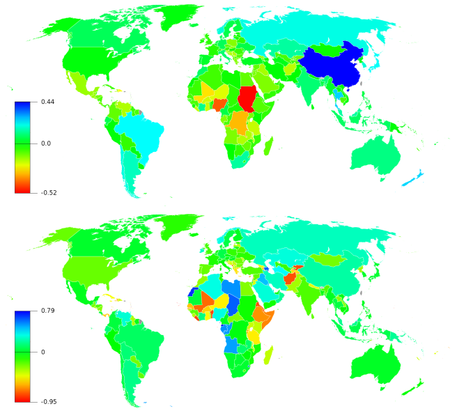
Fig. 20. World map of probabilities balance B_c = (P_c^* - P_c) / (P_c^* + P_c) determined for each of N_c = 227 countries in year 2008. Top panel: probabilities P_c^*, P_c are given by CheiRank and PageRank vectors; bottom panel: probabilities are computed from the trade volume of Export-Import (3). Names of countries can be find at [4].
