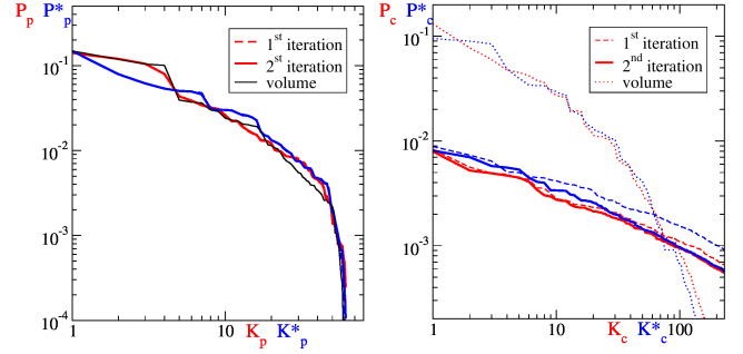
Fig. 3. Probability distributions of PageRank and CheiRank for products P_p(K_p) , P_p^*(K_p^*) (left panel) and countries P_c(K_c) , P_c^*(K_c^*) (right panel) in logarithmic scale for WTN from Fig. 2. Here the results for the 1 st and 2 nd GPVM iterations are shown by red (blue) curves for PageRank (CheiRank) with dashed and solid curves respectively. The probabilities from the trade volume ranking are shown by black curve (left) and dotted red and blue curves (right) for ImportRank and ExportRank respectively.
