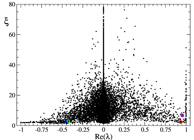
Fig. 15. Inverse participation ratio (IPR) \xi of all eigenstates of G as a function of the real part of the corresponding eigenvalue \lambda from the spectrum of Fig. 14. The eigenvalues marked by color circles are those from Fig. 14
