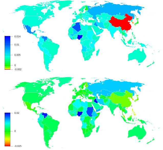
Fig. 22. Derivative of partial probability balance of product p defined as dB_{cp}/d\delta_{33} over petroleum price \delta_{33} for year 2008; here B_{cp} = (P_{cp}^* - P_{cp})/(P_c^* + P_c) and p = 72 ( 72 Electrical machinery ... from Table 1); the product balance of countries B_{cp} is determined from CheiRank and PageRank vectors (top panel) and from the trade volume of Export-Import (3) (bottom panel). Names of countries can be find at [4].
