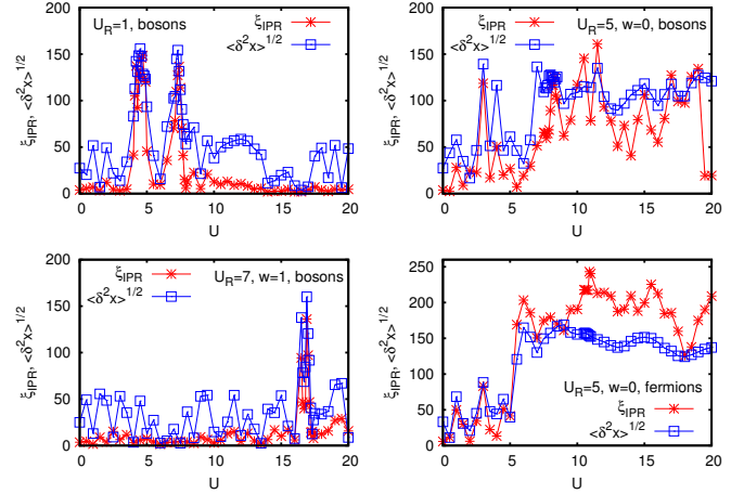
Fig. 1. Inverse participation ratio \xi_{\text{IPR}} and variance length \langle \delta^2 x \rangle^{1/2} = \langle (x - x_0)^2 \rangle^{1/2} of the time evolution two-particle state for system size N = 512 and iteration time t = 5120 (or t = 20480 for bottom left panel) versus interaction strength U . The initial state at t = 0 is localized either with both particles in the center position x_0 = N/2 (boson case) or antisymmetrized with one-particle in position x_0 and the other particle in position x_0 - 1 (fermion case). Both quantities have been calculated from an effective one-particle density without a center box of size 20% (with respect to system size). The different panels correspond to different cases of interaction range U_R , decay parameter w and boson/fermion case. Here \alpha/(2\pi) = (\sqrt{5} - 1)/2 and \beta = 0 .
