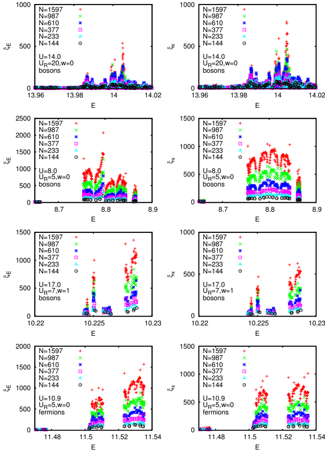
Fig. 11. Inverse participation ratio of eigenstates versus eigenvalue energy for the system sizes N = 144, 233, 377, 610, 987, 1597 and the same four cases with U_R > 1 as in Fig. 10 (see labels in panels for the values of the parameters U, U_R, w and boson or fermion case). The left column of panels correspond to the inverse participation ratio \xi_E in energy representation and the right column to the inverse participation ratio \xi_x in position representation.
