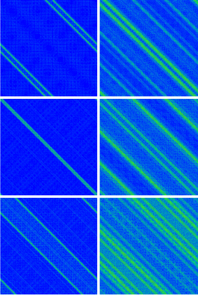
Fig. 13. Density plot of the three FIKS eigenstates in golden permutation Fourier representation with largest values of \xi_E for N = 610 , U_R = 1 , U = 4.5 (left column) or U = 7.8 (right column). The corresponding energy eigenvalues and values for both types of inverse participation ratios are: Top left: E = -3.09750 , \xi_E = 249.137 , \xi_x = 271.208 . Top right: E = -2.78586 , \xi_E = 211.058 , \xi_x = 194.241 . Center left: E = -3.09964 , \xi_E = 239.312 , \xi_x = 265.885 . Center right: E = -2.78599 , \xi_E = 200.958 , \xi_x = 176.454 . Bottom left: E = -3.09815 , \xi_E = 233.773 , \xi_x = 250.700 . Bottom right: E = -2.78593 , \xi_E = 190.171 , \xi_x = 193.885 .
