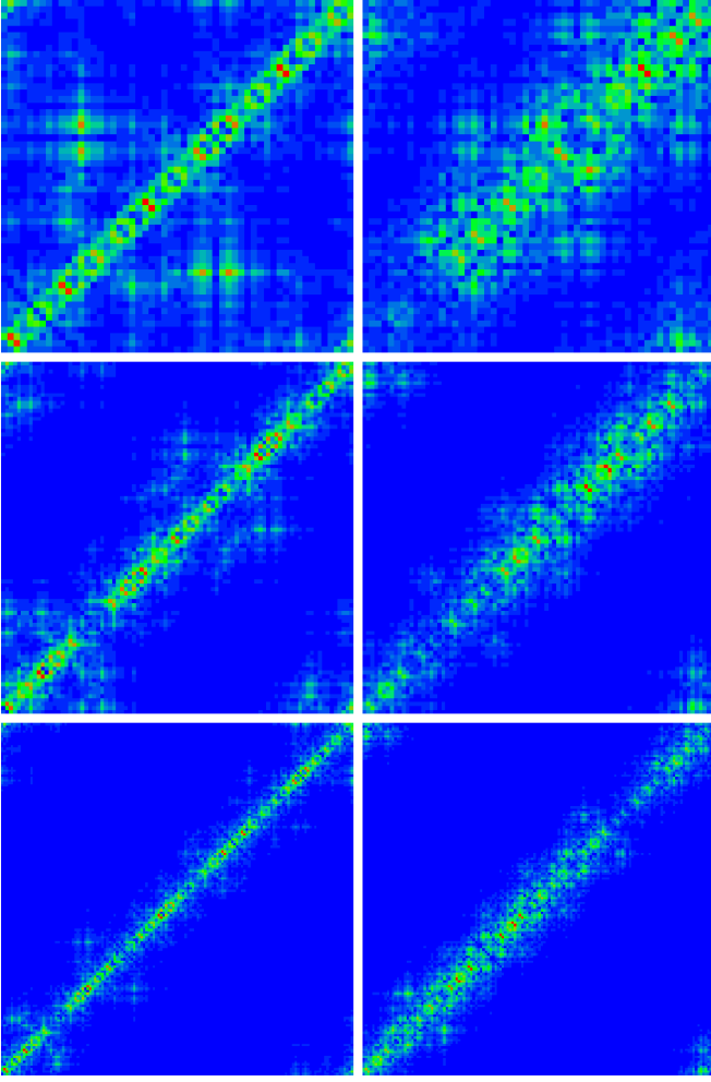
Fig. 4. Density plot of FIKS eigenstates with maximal value \xi_E for system size N = 55 (top panels), N = 89 (center panels), N = 144 (bottom panels), U_R = 1 and interaction strength U = 4.5 (left column) or U = 7.8 (right column). The corresponding energy eigenvalues and values for both types of inverse participation ratios are: Top left: E = -3.10334 , \xi_E = 22.756 , \xi_x = 30.794 . Top right: E = -2.75868 , \xi_E = 33.274 , \xi_x = 24.901 . Center left: E = -3.09588 , \xi_E = 50.742 , \xi_x = 49.867 . Center right: E = -2.78575 , \xi_E = 35.139 , \xi_x = 28.198 . Bottom left: E = 3.09966 , \xi_E = 61.373 , \xi_x = 63.353 . Bottom right: E = -2.78596 , \xi_E = 56.210 , \xi_x = 47.958 .
