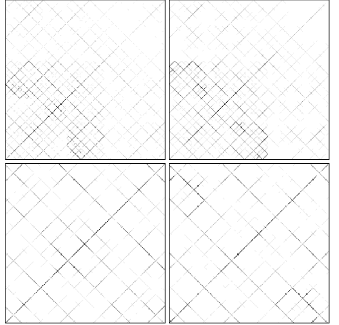
Fig. 14. Density plot of the FIKS eigenstates in non-interacting energy representation with the largest value of \xi_E for N = 233 (top panels) or N = 610 (bottom panels), U_R = 1 , U = 4.5 (left column) or U = 7.8 (right column). Black represents maximum, grey medium and white minimum values of the expansion amplitudes of the shown eigenstate with respect to non-interacting energy product eigenstates |\phi_\nu, \phi_\mu\rangle . The horizontal (vertical) axis corresponds to the index \nu ( \mu ) ordered with respect to increasing values of the corresponding one-particle energy \epsilon_\nu ( \epsilon_\mu ) of the first (second) particle. Top panels for N = 233 correspond to full eigenstates and bottom panels for N = 610 correspond to a zoomed region of size 200 \times 200 with left bottom corner at position x_1 = x_2 = 100 . The corresponding energy eigenvalues and values for both types of inverse participation ratios are: Top left: E = -3.09669 , \xi_E = 107.409 , \xi_x = 106.818 . Top right: E = -2.78569 , \xi_E = 117.697 , \xi_x = 102.577 . Bottom left: E = -3.09750 , \xi_E = 249.137 , \xi_x = 271.208 . Bottom right: E = -2.78586 , \xi_E = 211.058 , \xi_x = 194.241 .
