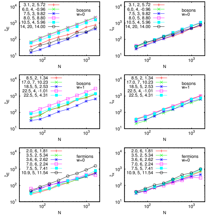
Fig. 12. Largest inverse participation ratio (for a given value of N ) of FIKS eigenstates versus system size N using all Fibonacci numbers between 55 and 1597 for selected cases of long range interactions (same data sets as in Table 3). The left column corresponds to the inverse participation ratio \xi_E in energy representation and the right column corresponds to the inverse participation ratio \xi_x in position representation. Top (center) panels correspond to the boson case with the decay parameter w = 0 ( w = 1 ). Bottom panels correspond to the fermion case with the decay parameter w = 0 . The three numbers in the color labels in the top left corner represent the interaction strength U , the interaction range U_R and the approximate energy eigenvalue E (for N = 1597 and the state with largest \xi_E ). Note that for a given value of N and set of interaction parameters the eigenstates with maximal \xi_x and maximal \xi_E may be different.
