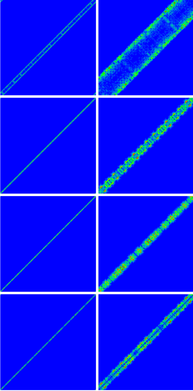
Fig. 10. Density plot of FIKS eigenstates for different cases of long range interaction U_R > 1 with maximal inverse participation ratio \xi_E in energy representation for N = 610 . The left column corresponds to the full eigenstate and the right column to a zoomed region of size 100 \times 100 with bottom left corner at position x_1 = x_2 = 200 . First row: U_R = 20 , w = 0 , U = 14 , boson case, energy eigenvalue E = 14.00502 , \xi_E = 263.410 , \xi_x = 350.519 . Second row: U_R = 5 , w = 0 , U = 8 , boson case, E = 8.79607 , \xi_E = 787.137 , \xi_x = 397.779 . Third row: U_R = 7 , w = 1 , U = 17 , boson case, E = 10.22864 , \xi_E = 635.918 , \xi_x = 307.585 . Fourth row: U_R = 5 , w = 0 , U = 10.9 , fermion case, E = 11.53294 , \xi_E = 535.618 , \xi_x = 360.478 .
