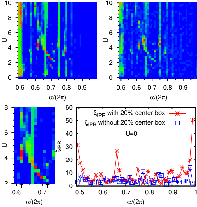
Fig. 21. Top panels : Density plot of the squared tail norm \|\psi_{\text{tail}}(t)\|^2 (left panel) or the inverse participation ratio computed without 20% center box (right panel) with horizontal axis representing the parameter \alpha/(2\pi) and vertical axis representing the interaction strength U using a time evolution state for system size N = 512 , iteration time t = 5120 , interaction range U_R = 1 and a localized initial state for t = 0 with both particles in the center position x_0 = N/2 . The bottom left panel shows a zoomed range with 0.6 \leq \alpha/(2\pi) < 0.75 and 2 \leq U \leq 8 of the top left panel. The two arrows indicate the value of the golden ratio \alpha/(2\pi) = (\sqrt{5} - 1)/2 \approx 0.618 and the value \alpha/(2\pi) = 266/369 \approx 0.721 used in the experiments of Ref. [21]. The bottom right panel shows the inverse participation ratio for U = 0 versus the parameter \alpha/(2\pi) and computed with (red crosses) and without (blue squares) the 20% center box. The maximal value is for the squared tail norm 0.12519 (for \alpha \approx 0.596 and U = 9.5 ) and for the the inverse participation ratio without 20% center box 188.68 (for \alpha \approx 0.753 and U = 4.5 ). The data of this figure are obtained with \beta = (\sqrt{5} - 1)/2 (and not \beta = 0 as the data of Fig. 1 and Table 1 in Sec. 4).
