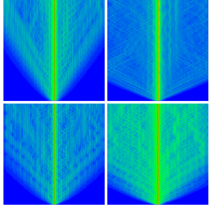
Fig. 3. Density plot for the time dependence of one-particle density from the time evolution state with x -position ( 0 \leq x < 512 ) corresponding to the horizontal axis and time t ( 0 \leq t \leq 5120 or 0 \leq t \leq 20480 for bottom left panel) corresponding to the vertical axis. The four panels correspond to the same parameter values of U , U_R , w and boson/fermion cases as in four panels of Fig. 2.
