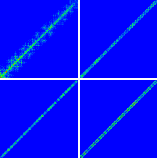
Fig. 2. Density plot of time evolution state for t = 5120 (or t = 20480 for bottom left panel), system size N = 512 , the four cases of Fig. 1 and with a value of U corresponding to strongest delocalization: U = 4.5 , U_R = 1 , boson case (top left panel), U = 8 , U_R = 5 , w = 0 , boson case (top right panel), U = 16.9 , U_R = 7 , w = 1 , boson case (bottom left panel), U = 10.9 , U_R = 5 , w = 0 , fermion case (bottom right panel). We show only zoomed region of size 205 \times 205 with left bottom corner at position x_1 = x_2 = 307 which corresponds to the right/top boundary of the 20% center box. The colors indicate red for maximum, green for medium and blue for minimum values (same distribution of colors in other figures of density plots).
