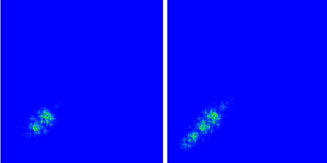
Fig. 20. Density plot of two selected eigenstates for U = 4.5 , U_R = 1 and for the rational approximations of \alpha_2/(2\pi) . The corresponding system sizes, energy eigenvalues and values for both types of inverse participation ratios are: Left: N = 369 , E = -2.21758 , \xi_E = 11.378 , \xi_x = 21.029 (2nd largest value of \xi_E and largest value of \xi_x for this system size and approximate energy). Right: N = 1605 , E = -2.21949 , \xi_E = 16.367 , \xi_x = 26.748 (largest value of \xi_E for this system size and approximate energy). The left panel shows the full state of size 369 \times 369 and the right panel a zoomed region of size 369 \times 369 with left bottom corner at position x_1 = x_2 = 0 and outside the zoomed range no data points different from blue (for zero amplitude) are visible.
