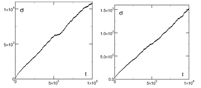
Fig. 11. Time dependence of the second moment \sigma(t) = \langle (x_1)^2 + (x_2)^2 \rangle / 2 averaged over 500 orbits taken in a close vicinity to each other at \lambda = 2.5, U = 6, E \approx -0.856 (left panel) and \lambda = 4.5, U = 12, E \approx 0.129 (right panel). The fit gives the diffusion rate \sigma = Dt + \text{const.} with D = 0.0106 \pm 3.7 \times 10^{-6} (left panel) and D = 0.00143 \pm 3.8 \times 10^{-7} (right panel).
