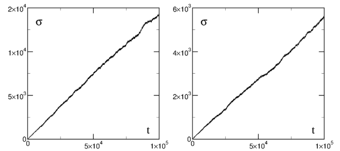
Fig. 4. Time dependence of the second moment \sigma(t) = \langle ((x_1)^2 + (x_2)^2)/2 \rangle averaged over 10^3 orbits taken in a vicinity of trajectories of Figure 2 at \lambda = 2.5 , U = 6 , E \approx 1.884 (left panel) and \lambda = 4.5 , U = 12 , E \approx 3.876 (right panel). The fit gives the diffusion rate \sigma = Dt + \text{const.} with D = 0.143 \pm 3.2 \times 10^{-5} (left panel) and 0.0543 \pm 1.4 \times 10^{-4} (right panel).
