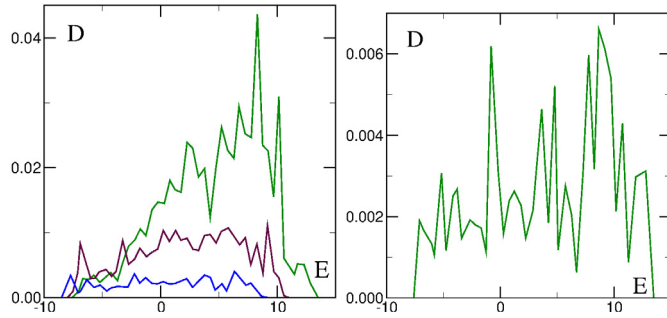
Fig. 10. Dependence of diffusion rate D on TIP energy E for same trajectories as in Figure 9 at same parameters and colors with \lambda = 2.5 (left panel), \lambda = 4.5 (right panel).
