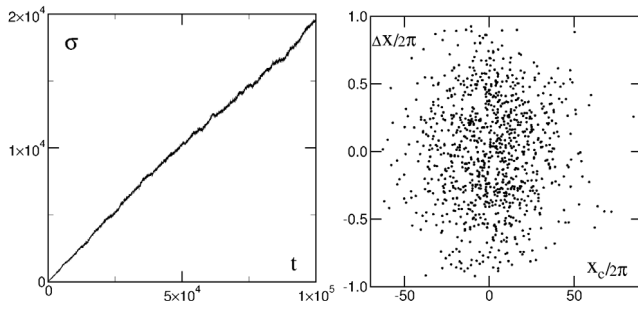
Fig. 8. Left panel: time dependence of the second moment \sigma(t) = \langle ((x_1)^2 + (x_2)^2)/2 \rangle for the short range interaction model (6); data are averaged over 10^3 orbits taken in a chaotic component in a vicinity of energy E = 3.32 at \lambda = 2.5 , U = 6 , the fit gives the diffusion growth \sigma = Dt + \text{const.} with D = 0.189 \pm 6 \times 10^{-5} . Right panel: the distribution of \Delta x = (x_2 - x_1) and x_c = (x_1 + x_2)/2 is shown for orbits of left panel at t = 10^5 .
