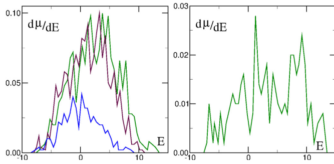
Fig. 9. Dependence of differential measure of diffusive trajectories d\mu/dE on TIP energy E in the 2D Harper model for: \lambda = 2.5 and U = 1 (blue), 3 (brown), 6 (green) with corresponding total measure \mu = 0.265, 0.796, 0.893 (left panel); \lambda = 4.5 and U = 6 (green) with corresponding total measure \mu = 0.217 , for U = 3; 1 the measure is small being respectively \mu = 0.023; 0 and these data are not shown (right panel). Data are obtained from N = 10^3 trajectories homogeneously distributed in the phase space and iterated till time t = 4 \times 10^5 ; averaging is done over energy interval \Delta E = 0.5 .
