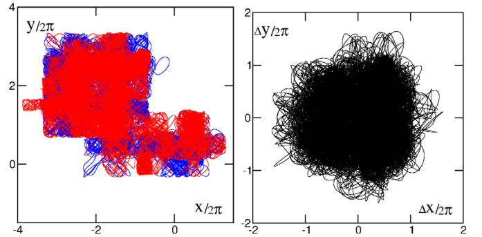
Fig. 12. Example of dynamics of one trajectory from Figure 11 (left panel at \lambda = 2.5, U = 6, E = -0.856 ) for time t \leq 10^4 is shown on (x, y) plane with first particle in blue and second particle in red colors (left panel); the evolution of distance between particles \Delta x = x_2 - x_1, \Delta y = y_2 - y_1 is shown on right panel.
