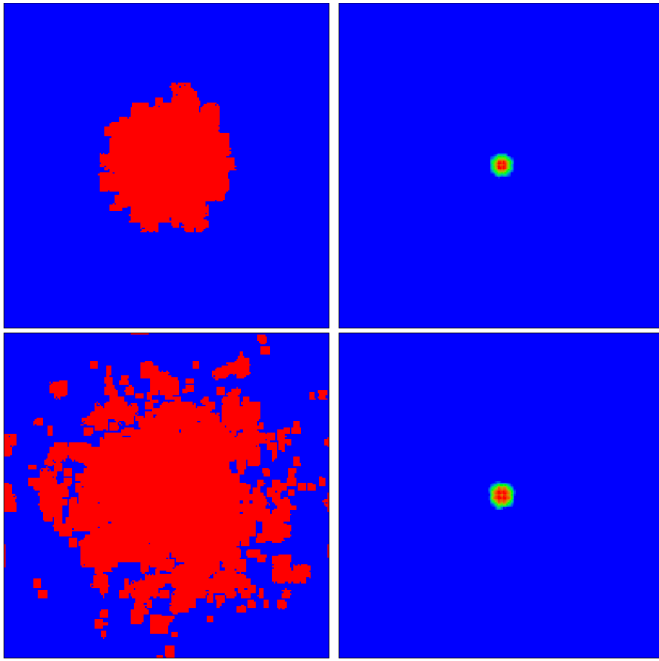
Fig. 13. Density distribution of TIP at parameters \lambda = 2.5 , U = 6 , E = -0.856 averaged over 10^3 trajectories. Left column: density of charge (sum over each particle) in the plane (x/2\pi, y/2\pi) at time t = 10^4 at top panel and t = 10^5 at bottom panel (average over time interval \delta t = 10^3 ); right column: density distribution over distance between particles \Delta x/2\pi = (x_2 - x_1)/2\pi , \Delta y/2\pi = (y_2 - y_1)/2\pi at time t = 10^4 at top panel and t = 10^5 at bottom panel (average over all times from zero to t ). The panels show the squares -16 \leq x/2\pi, y/2\pi \leq 16 (left), -16 \leq \Delta x/2\pi, \Delta y/2\pi \leq 16 (right); at t = 0 TIP are located in one cell; color changes from blue (zero) to red (maximum).
