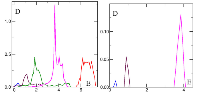
Fig. 7. Dependence of diffusion rate D on TIP energy E for same trajectories as in Figure 6 at same parameters and colors with \lambda = 2.5 (left panel), \lambda = 4.5 (right panel).
