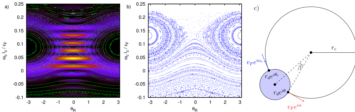
FIG. 1: Left panel (a): density of Husimi function at the disc radius r = r_d shown by color (maximum for yellow/white; minimum zero for violet/black), Poincaré section for classical Hamiltonian dynamics of (2) is drawn at the moment of collision with disc and is shown by green dots; here J = 2.7 , r_d/\ell_B = 1 , qE_{ac}\ell_B/\hbar\omega_c = 0.3 at energy \epsilon_F/\hbar\omega_c \approx 40 . Middle panel (b): classical Poincaré section of the collision map (5) at parameters of panel (a). Right panel (c): geometry of collision.
