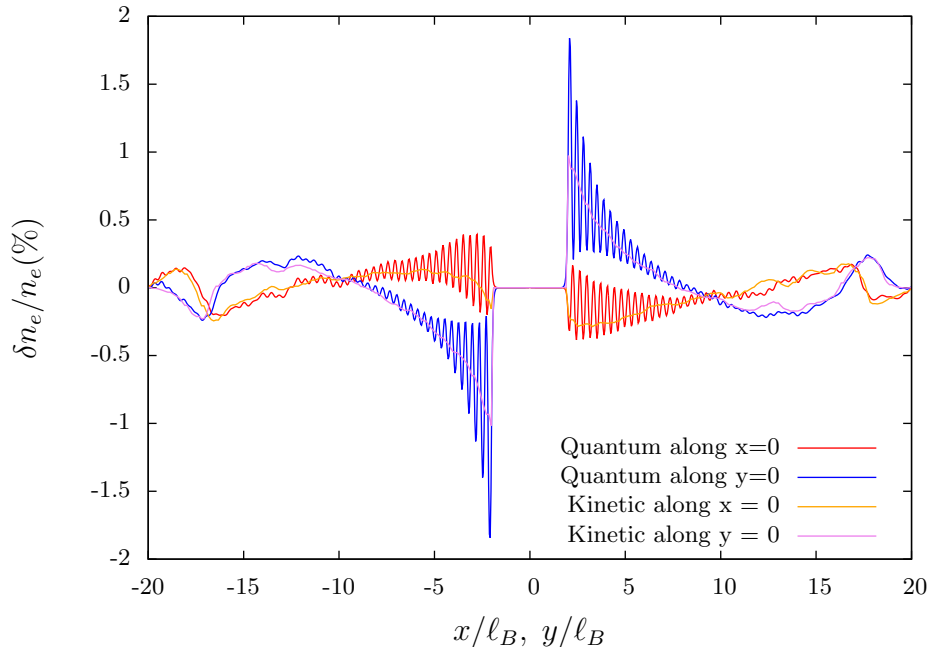
FIG. 3: Charge density \rho(x, y) dependence on x (at y = 0 ) and on y (at x = 0 ) obtained from the quantum master equation and the classical kinetic equation presented in the rotation frame. Here the system parameters are the same as for the repulsive case in Fig. 2 with J = 2.7 for r_d/\ell_B = 2 at qE_{ac}\ell_B/\hbar\omega_c = 0.1 and \epsilon_F/\hbar\omega_c = 40 with a relaxation time \omega_c\tau = 10 .
