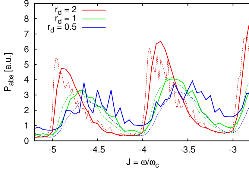
Supplementary Figure S3: Dependence of the microwave absorption \mathcal{P}_{abs} on J (arbitrary units) for different values of impurity radius r_d obtained from the quantum master equation Eq. (S92) (full curves) and the classical kinetic equation Eq. (S93) (dashed curves). Here U_{disc} = 2\epsilon_F , qE_{ac}\ell_B/\hbar\omega_c = 0.1 and \omega_c\tau = 100 . The semiclassical curves reproduce correctly the results from the quantum master equation. For r_d/\ell_B = 0.5 additional fluctuations appear in the quantum calculation around an average lineshape which is still well describe by the semiclassical calculation. We attribute those to interference effects which become more pronounced when the size of the impurity becomes closer to the Fermi wavelength. In a real sample such fluctuations would probably be suppressed by ensemble average leaving only an average average value which would correspond to the semiclassical result.
