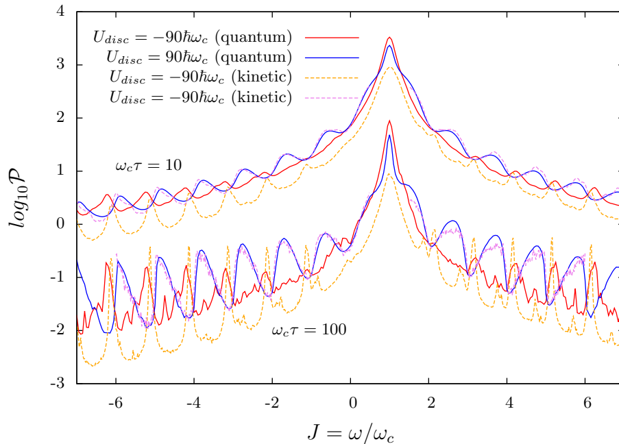
FIG. 2: Absorption power \mathcal{P} (in arbitrary units) is shown as a function of J = \omega/\omega_c for r_d/\ell_B = 2 at qE_{ac}\ell_B/\hbar\omega_c = 0.1 and \epsilon_F/\hbar\omega_c = 60 . Data are shown for two relaxation times with \omega_c\tau = 10, 100 (different signs of J correspond to different signs of circular polarization). Quantum results are obtained from the master equation on the density matrix, they are compared with classical results from the kinetic equation. An excellent agreement between quantum and classical results is observed for a repulsive potential. For an attractive potential the agreement is only qualitative the kinetic equation giving the same phase of microwave absorption oscillations as the quantum calculation.
