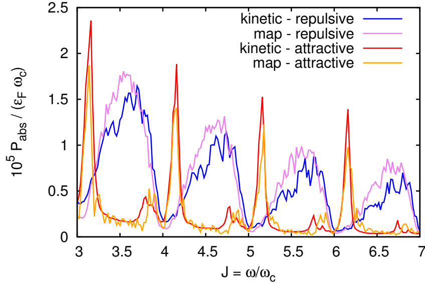
Supplementary Figure S2: Dependence of the average absorbed microwave power P_{abs} for electrons colliding with an impurity for parameters: qE_{ac}/(m\omega v_F) = 0.013 , r_d/R_c = 0.13 , \omega_c\tau = 100 , U_{disc} = \pm 2\epsilon_F , a good agreement is observed between results from the kinetic equation and from the collision map S77.
