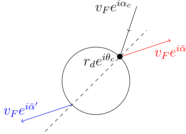
Supplementary Figure S1: Geometry of reflection during collision with a disc in case of attractive and repulsive potentials.
