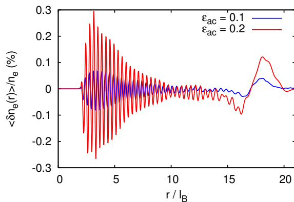
FIG. 7: Relative variation of the time averaged electron charge density \langle \delta n_e(r) \rangle / n_e induced by a microwave irradiation, as a function of radial distance r from the impurity. The results are shown two microwave fields \epsilon_{ac} = 0.1 and 0.2 ( \epsilon_{ac} = qE_{ac} \ell_B / \hbar \omega_c ). Other parameters are as in Fig. 3 ( r_d/\ell_B = 2 , E_F/\hbar \omega_c = 40 ). \omega_c \tau = 100
