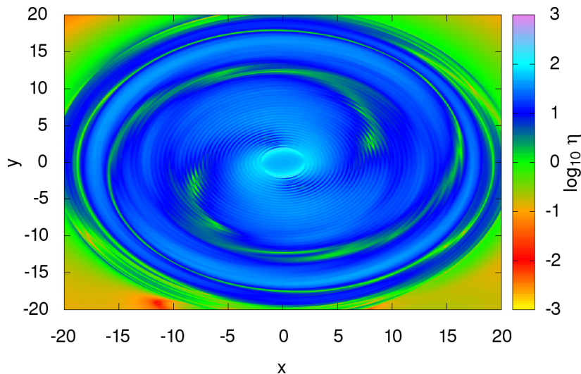
FIG. 5: Variation of the enhancement factor E_{ee}/E_{ac} of the amplitude of effective field acting on an electron due to the density variation in (x, y) plane (see Fig. 4 left panel) induced by the external microwave field. The results, shown in the rotating frame, are obtained from the quantum master equation and the relations given by Eq.(12).
