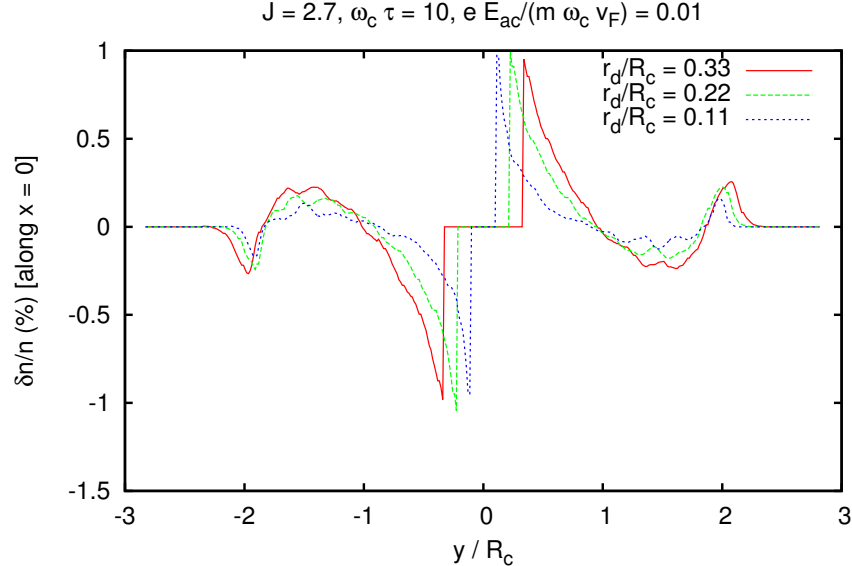
Supplementary Figure S5: Dependence of \delta n_e(x=0, y)/n_e on y/R_c for different impurity diameters, results are shown for the kinetic equation calculation.
