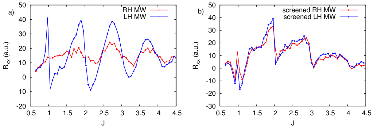
FIG. 6: Dependence of resistivity R_{xx} (in arbitrary units a.u.) on J = \omega/\omega_c . Left panel: the case of initial external microwave field; right panel: the case of screened renormalized field acting on a length-scale r_{eff}/R_c = 0.3 . The results are obtained from the numerical simulation of classical Hamiltonian dynamics of electrons in presence of impurities with Gaussian potential U_{amp} \exp(-r^2 r_d^{-2}) with a density n_i r_d^2 = 10^{-3} an amplitude U_{amp}/\epsilon_F = 1.5 and a characteristic radius r_d \omega/v_F = 0.1 .
