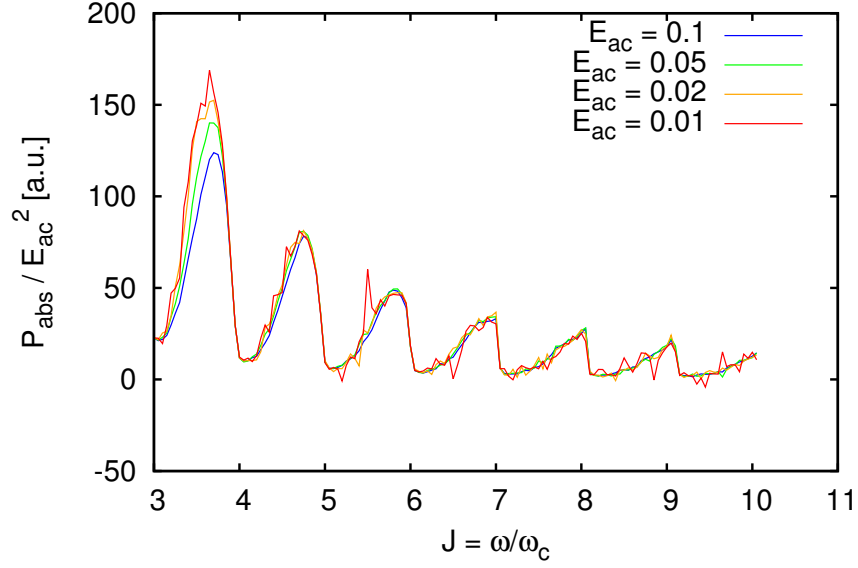
Supplementary Figure S4: Scaling dependence of the microwave absorption \mathcal{P}_{abs} rescaled by incident microwave power \propto E_{ac}^2 on J (arbitrary units) for different amplitudes of microwave field E_{ac} . The results are obtained from the quantum master equation Eq. (S92) for a repulsive impurity potential ( U_d = 90\hbar\omega_c ) at \omega_c\tau = 100 and 0.01 \leq E_{ac} \leq 0.1 . The data show that the scaling \mathcal{P}_{abs} \propto E_{ac}^2 is highly accurate. At the lowest microwave powers the data become more noisy and start to show individual resonances, we think that the sharp peaks comes from contributions of individual levels trapped around the impurity that lead to sharp resonances due to the high \omega_c\tau = 100 value. At higher microwave power the individual resonances are broadened giving the semiclassical absorption curve.
