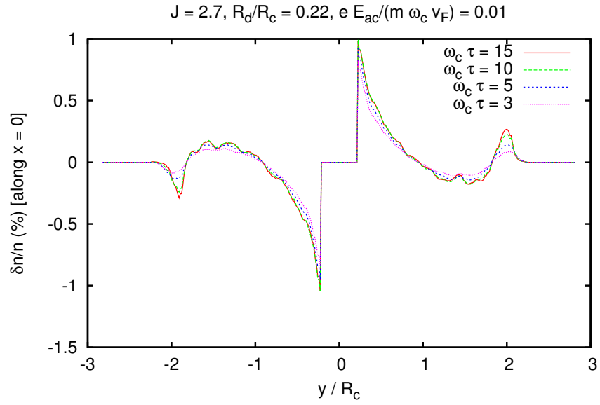
Supplementary Figure S7: Dependence of \delta n_e(x=0, y)/n_e on y/R_c for different values of \omega_c \tau .
