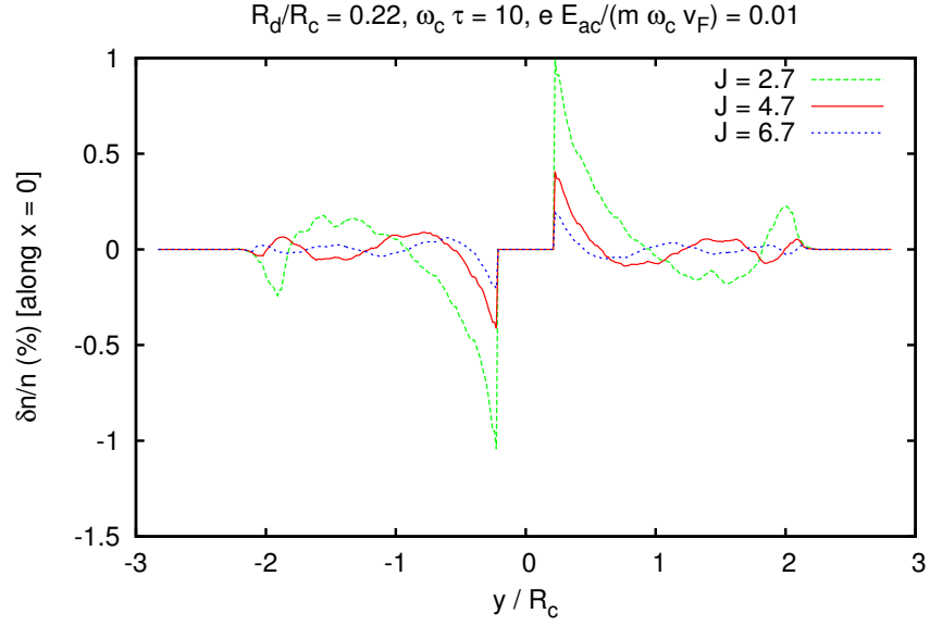
Supplementary Figure S6: Dependence of \delta n_e(x=0, y)/n_e on y/R_c for different values of J = \omega/\omega_c .
