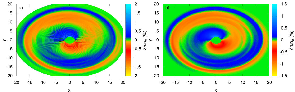
FIG. 4: Relative charge density variation \rho(x, y) = \delta n/n_0 (expressed in percent) shown in (x, y) plane in the rotation frame where a microwave field is directed along x -axis. Left panel shows the results of quantum simulations with the master equation, left panel show the results of the classical kinetic equation. The parameters are the same as in Fig. 3.
