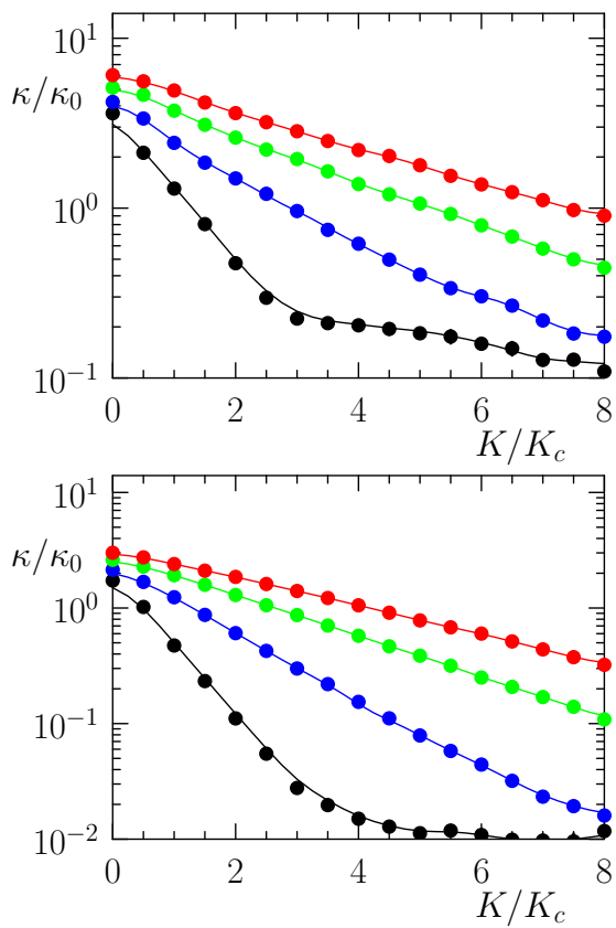
FIG. S.3: Dependence of the rescaled heat conductivity of the atom chain \kappa/\kappa_0 on the rescaled potential amplitude K/K_c at different rescaled temperatures T/K_c . The rescaled parameters are the same as in Fig. S.2. Here \sigma_0 = \nu/(2\pi\eta) , \kappa_0 = \sigma_0 K_c .
