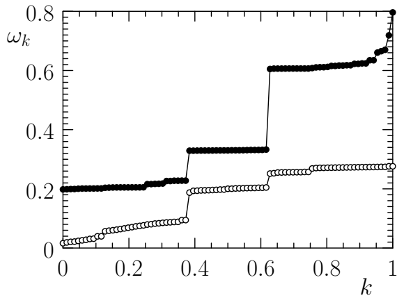
FIG. 2: Phonon spectrum \omega(k) for K = 0.02 (open circles) and K = 0.1 (full circles) for \nu = N/L = 89/55 .
