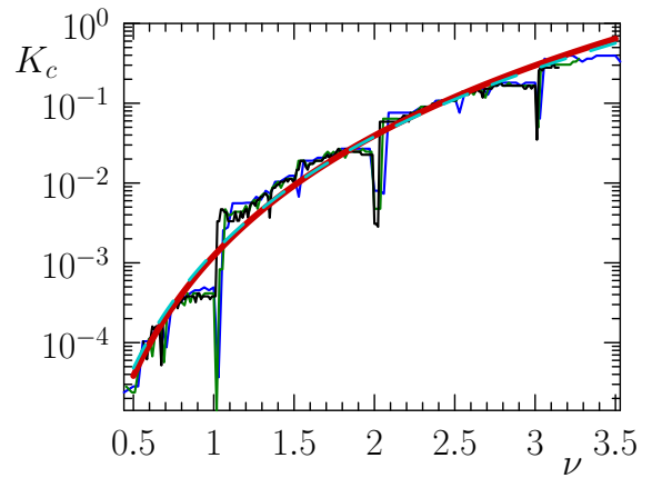
FIG. 3: Dependence of the Aubry transition critical threshold K_c on the atomic density \nu shown for different chain lengths L = 34 (blue curve), 55 (green curve) and 89 (black curve). The red full curve shows the theoretical dependence (3), the dashed cyan curve shows the fit with K_c = 0.0137(\nu/\nu_g)^\alpha , \nu_g = 1.618 and \alpha = 4.82 \pm 0.08 .
