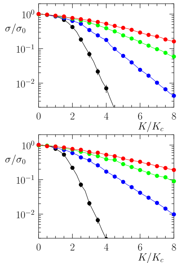
FIG. S.2: Dependence of the rescaled conductivity of the atom chain \sigma/\sigma_0 on the rescaled potential amplitude K/K_c at different rescaled temperatures T/K_c . Top panel: T/K_c = 0.25 (black curve), 1 (blue curve), 2 (green curve), 3 (red curve), curves from bottom to top, \nu = 34/21 \approx 1.618 , K_c = 0.019 ; bottom panel: same values of T/K_c with the same order of curves, \nu = 55/21 \approx 1.618 , K_c = 0.14 . Here \sigma_0 = \nu/(2\pi\eta) .
