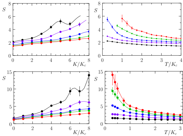
FIG. 4: Dependence of the Seebeck coefficient S on the rescaled potential amplitude K/K_c (left column) and temperature T/K_c (right column) for N/L = 34/21 = \nu \approx 1.618 (top row) and N/L = 55/21 = \nu \approx 2.618 (bottom row). Left: color curves show the cases T/K_c = 0.5, 1, 2, 3, 4 for N/L = 34/21 and T/K_c = 0.3, 0.8, 1.3, 1.6, 2.3 for N/L = 55/21 (black, violet, blue, green, red from top to bottom curves). Right: K/K_c = 0, 2, 4, 6, 8 for N/L = 34/21 and N/L = 55/21 (black, violet, blue, green, red from bottom to top curves). Here, K_c = 0.019 for \nu = 34/21 and K_c = 0.14 for \nu = 55/21 .
