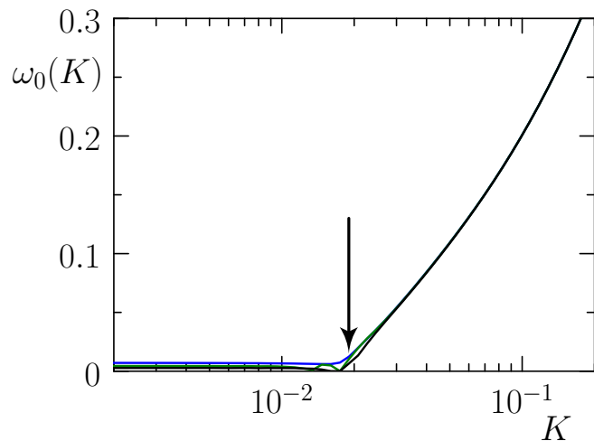
FIG. S.1: Dependence of the lowest phonon frequency \omega_0 on K for the lattice with N dipole atoms in L lattice periods at density \nu \approx 1.618 : N/L = 55/34 (blue curve), 89/55 (green curve), 144/89 (black curve); arrow marks the point of the Aubry transition at K_c = 0.019 defined as it is described in the text.
