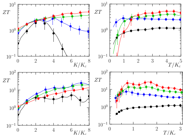
FIG. S.5: Dependence of ZT on the rescaled potential amplitude K/K_c (left column) and on the rescaled temperature T/K_c (right column) for N/L = 34/21 = \nu \approx 1.618 (top row) and N/L = 55/21 = \nu \approx 2.618 (bottom row). Left: color curves show the cases T/K_c = 0.5, 1, 2, 3, 4 for N/L = 34/21 and T/K_c = 0.3, 0.8, 1.3, 1.6, 2.3 for N/L = 55/21 (black, violet, blue, green, red from top to bottom curves). Right: K/K_c = 0, 2, 4, 6, 8 for N/L = 34/21 and N/L = 55/21 (black, violet, blue, green, red from bottom to top curves). Here K_c = 0.019 for \nu = 34/21 and K_c = 0.14 for \nu = 55/21 .
