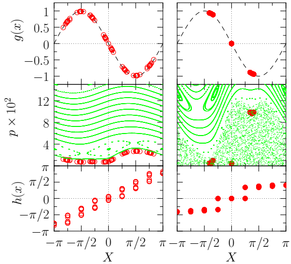
FIG. 1: Functions related to the dynamical map obtained from the ground state equilibrium positions x_i of atoms at K = 0.02 (open circles, left column) and K = 0.1 (full circles, right column). Panels show: the kick function g(x) (top); the map (2) phase space (p, x) with g(x) = -\sin x (green points) and actual atom positions (red circles) (middle); the hull function h(x) (bottom). The atom positions are shown via the hull function h(x) = (x_i + \pi)[\text{mod } 2\pi] - \pi versus x = (2\pi(i - 1)/\nu + \pi)[\text{mod } 2\pi] - \pi ; the positions of the two atoms at the chain ends are fixed. Here we have N = 89 atoms and L = 55 periods, \nu = 89/55 .
