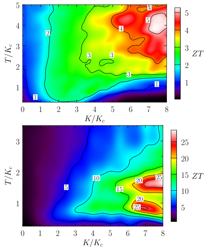
FIG. 5: Color map of the figure of merit ZT values for density \nu = N/L = 34/21 \approx 1.618 (top panel) and \nu = N/L = 55/21 \approx 2.618 (bottom panel); numbers mark isocontour values of ZT ; K_c values are as in Fig. 4.
