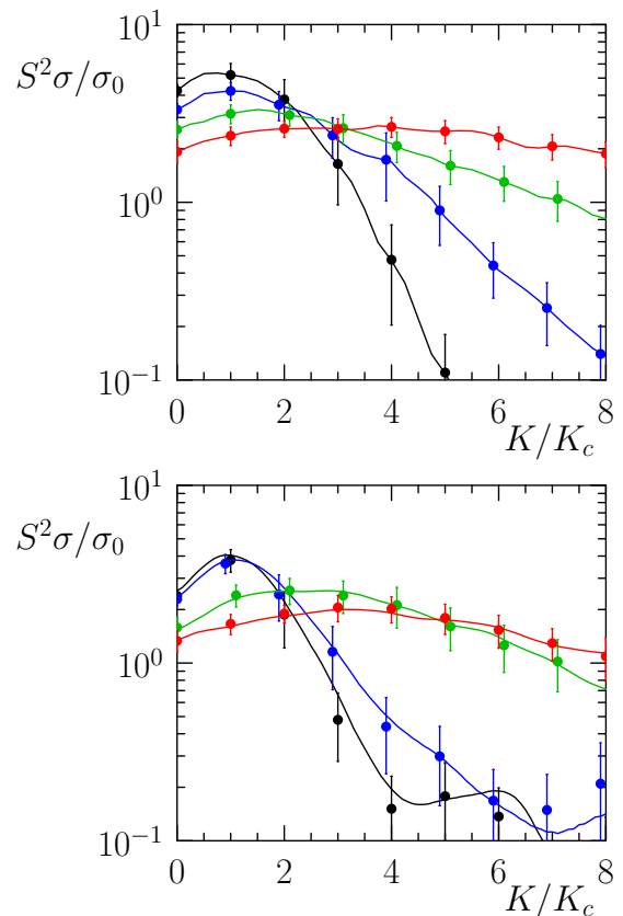
FIG. S.6: Dependence of the power factor P_S = S^2\sigma/\sigma_0 on system parameters. Top panel: \nu = N/L = 34/21 , T/K_c = 0.25, 1, 2, 4.25 (black, blue, green, red colors), K_c = 0.019 . Bottom panel: \nu = N/L = 55/21 , T/K_c = 0.25, 0.5, 1.5, 2.5 (black, blue, green, red colors), K_c = 0.14 .
