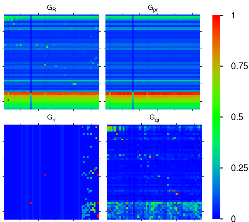
Figure 2. Color density plots of the matrix components G_R , G_{pr} , G_{rr} , G_{qr} for the group of Table 1; the x -axis corresponds to the first (row) index (increasing values of K_g ) from top to down) and the y -axis corresponds to the second (column) index of the matrix (increasing values of K_g from left to right). The outside ticks indicate multiples of 10 of K_g . The numbers in the color bar correspond to \sqrt{|g|/g_{\max}} , with g being the value of the matrix element and g_{\max} being the maximum value. In order to increase the visibility for the cases of G_R , G_{rr} , G_{qr} , the maximum value has been reduced (saturated) to the value of the third largest value of g for each case, and the cells corresponding to the first and second largest values are reduced to the saturation value. In particular, G_R(45, 15) ( G_R(46, 13) ) has been reduced from 0.876387 (0.297512) to G_R(49, 3) = 0.208777 ; G_{rr}(45, 16) ( G_{rr}(29, 24) ) has been reduced from 0.850004 (0.121432) to G_{rr}(29, 54) = 0.019322 (same third value also for the other three cells in column 54); G_{qr}(49, 3) ( G_{qr}(40, 41) ) has been reduced from 0.240629 (0.062024) to G_{qr}(46, 32) = 0.041108 . For the matrix G_{qr} , there are some negative values, and here, we show their absolute values (see text).
