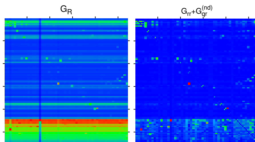
Figure 8. Color density plots of G_R and G_{rr} + G_{qr}^{(nd)} for the bifunctional Ising MetaCore network and the extended group of 108 nodes by attribution of labels (+) and (−) to each node of Table 1. The matrix plot style is similar to in Figure 2, with outside ticks indicating multiples of 20 of the index values. The color bar is as in Figure 2 with the same translation of colors to matrix values. The saturation value is, for both panels, the sixth largest value for each matrix, and larger values are reduced to this value. The strongest cell values are reduced from 0.437575 (0.424939) to 0.101874 (0.060717) for G_R ( G_{rr} + G_{qr}^{(nd)} ).
