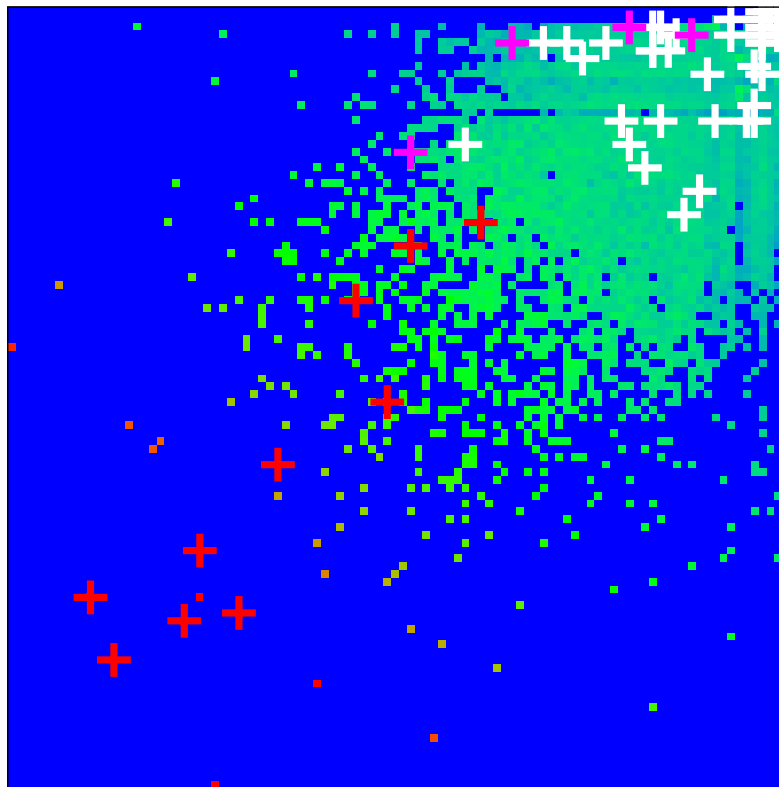
Figure 1. Density of nodes W(K_M, K_M^*) on PageRank–CheiRank plane ( K_M, K_M^* ) averaged over 100 \times 100 logarithmically equidistant grids for 0 \leq \ln K_M, \ln K_M^* \leq \ln N ( 1 \leq K_M, K_M^* \leq N = 40,079 ); the density is averaged over all nodes inside each cell of the grid, the normalization condition is \sum_{K_M, K_M^*} W(K_M, K_M^*) = 1 . Color varies from blue at zero value to red at maximal density value. In order to increase the visibility, large density values have been reduced to (saturated at) 1/16 of the actual maximum density and typical green cells correspond to density values of \sim 1/2^8 of the (reduced) maximum density. The x -axis corresponds to \ln K_M and the y -axis to \ln K_M^* with K_M ( K_M^* ) being the global PageRank (CheiRank) index for the full MetaCore network. The crosses mark the positions of the 54 proteins of Table 1 with colors: red for the X-proteins, pink for the TGF- \beta subgroup, and white for the up- and down-protein subgroups.
