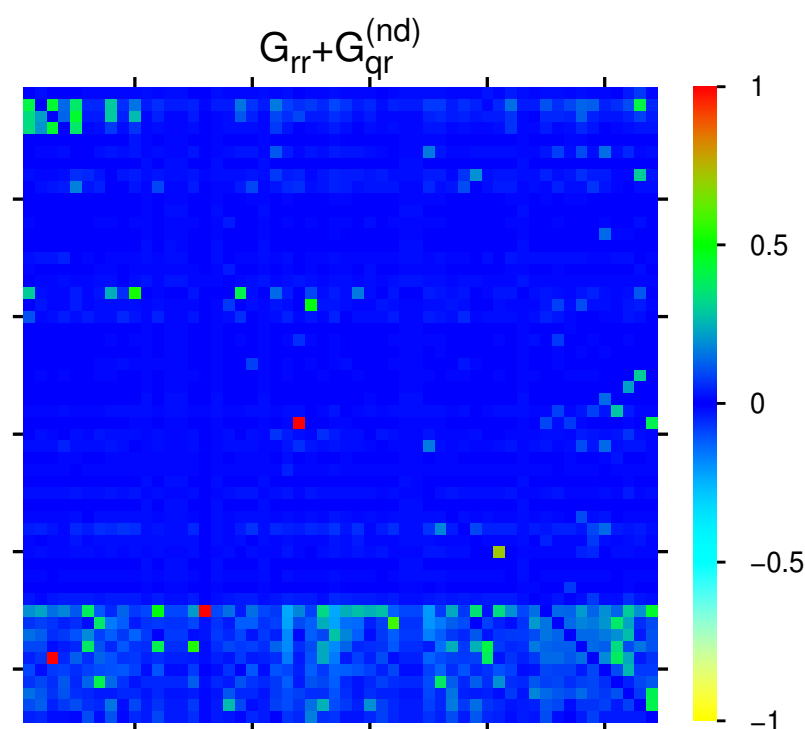
Figure 3. Color density plot G_{rr} + G_{qr}^{(nd)} for the group of Table 1. The matrix element at (45, 16) ((49, 3)) has been reduced from 0.849861 (0.240632) to the value 0.121433 at (29, 24); a few matrix elements of G_{rr} + G_{qr}^{(nd)} have negative values visible as cyan color (see text). The numbers in the color bar correspond to \text{sgn}(g) \sqrt{|g|/g_{\max}} , with g being the value of the matrix element and g_{\max} being the maximum value.
