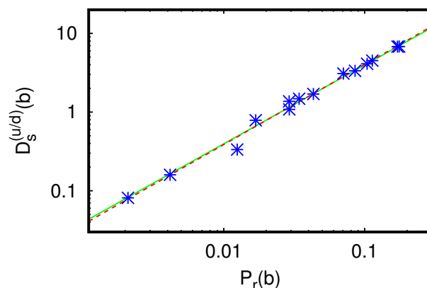
Figure A5. Dependence of the sum of sensitivities D_s^{(u/d)}(b) from Table 3 on the (local) PageRank probability P_r(b) ; the straight green line shows the fit dependence D_s^{(u/d)}(b) = \eta P_r(b) with the obtained numerical value \eta = 39.5 \pm 1.4 ; the dashed red line corresponds to the power law fit D_s^{(u/d)}(b) = \tilde{\eta} [P_r(b)]^\kappa with \tilde{\eta} = 41.9 \pm 4.3 and \kappa = 1.017 \pm 0.028 .
