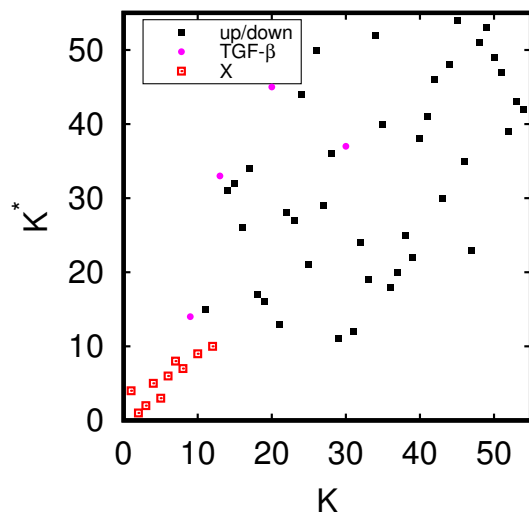
Figure A1. Positions of the 54 proteins of Table 1 in the local PageRank–CheiRank. Note that these positions are identical to the positions of Figure 7 and the corresponding K, K^* values are given in the 3rd and 4th column of Table 1. Pink full circles correspond to the subgroup of TGF- \beta nodes, full black boxes correspond to the subgroups of up- and down-proteins and red squares correspond to the subgroup of X-proteins.
