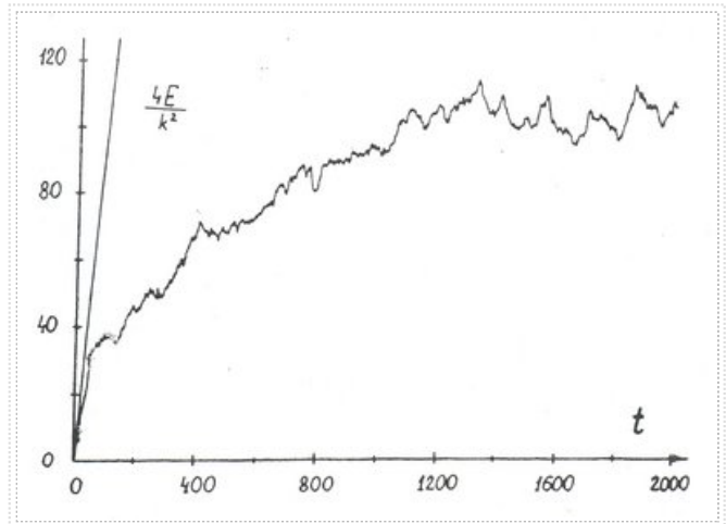
Figure 4: Dependence of rescaled rotator energy E/(k^2/4) on time t for K = kT = 5 , \hbar = 0.25(k = 20, T = 0.25) the full curve shows numerical data and the straight line gives the diffusive energy growth in the classical case (from [23]).
