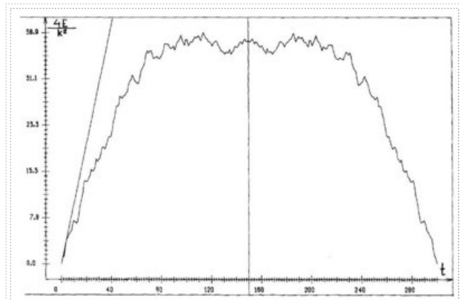
Figure 7: Same as in Fig.6 but for the quantum map (2) with K = 5, \hbar = 0.25 , the straight line shows the classical diffusion; time reversal is performed at the moment t = 150 marked by the vertical line, numerical simulations are done on the same computer BESM-6, in addition random quantum phases 0 < \Delta\phi < 0.1 are added for quantum amplitudes in momentum representation at the moment of time reversal (from [46]).
