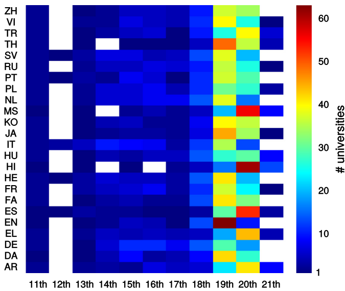
Fig. 13. Distribution over foundation century for PageRank top 100 universities of each Wikipedia edition. Dark red color corresponds to maximum with 63 for EN in 19th century, dark blue color corresponds to one university, white color represents zero.
