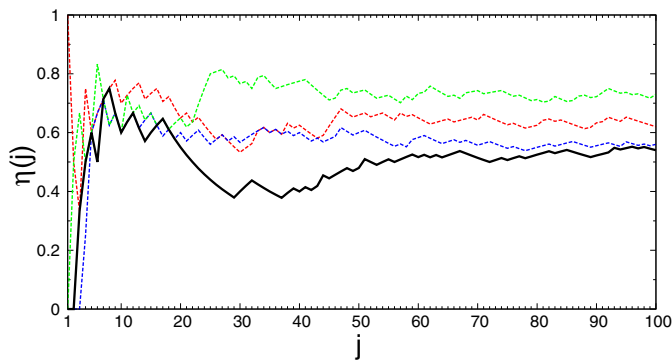
Fig. 2. Overlap \eta(j) = j_c/j between: W2RWU and ARWU (black curve), W2RWU and WPRWU (red dashed curve), W2RWU and WCRWU (blue dashed curve), WPRWU and WCRWU (green dashed curve). Here j is the rank index of both compared ranks, j_c is number of common items among j ranks.
