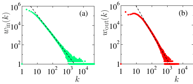
Fig. 1. (Color online) Distribution w_{in,out}(k) of incoming (a) and outgoing (b) links k for N = 3\,282\,257 Wikipedia English articles. The straight dashed fit line shows the slope with \mu_{in} = 2.09 \pm 0.04 (a) and \mu_{out} = 2.76 \pm 0.06 (b).
