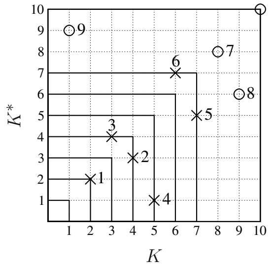
Fig. 7. A toy example illustrating the functioning of 2DRank algorithm of node ranking in K, K^* plane: square size k \times k is regularly increase in size k \rightarrow k + 1 , nodes appearing on edges of this square at each step are included in the listing K_2 of 2DRank (crosses), first on right edge, then on top edge; nodes outside of the square (circles) are included in the listing K_2 at later stage. Numbers near symbols give K_2 values of 2DRank.
