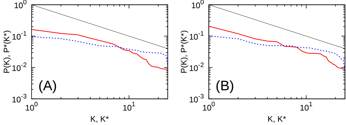
Figure S1. Dependence of probabilities of PageRank P (red) and CheiRank P^* (blue) on corresponding indexes K and K^* . The probabilities are obtained from the network shown in Fig.7 for corresponding panels (A),(B). The straight lines indicate the Zipf's law P \sim 1/K ; P^* \sim 1/K^* .
