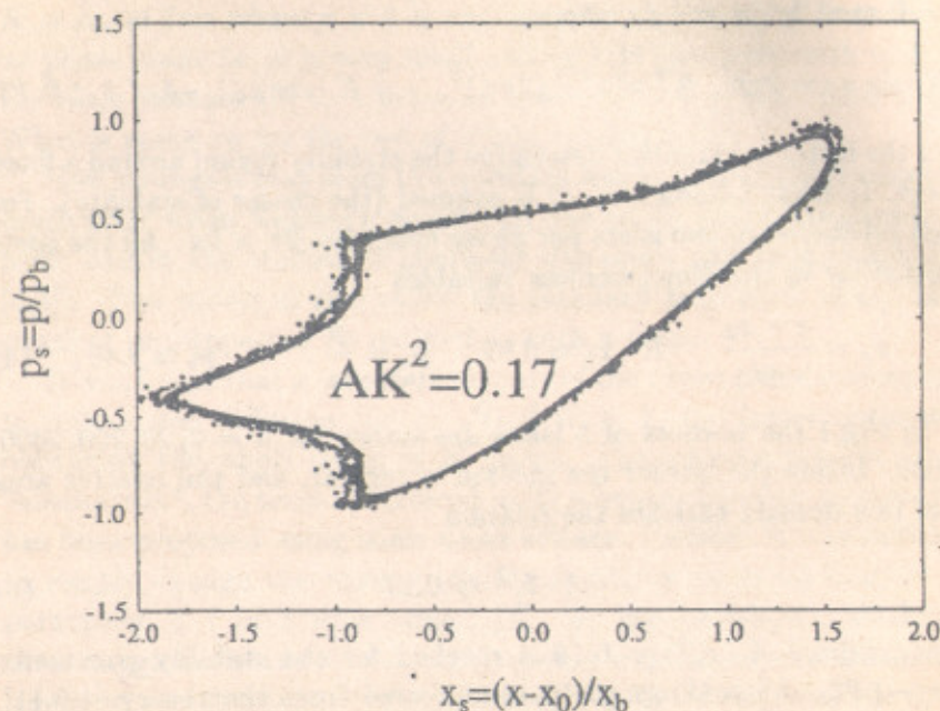
Figure 1: Universal border of microtron domains in dimensionless variables (4): n = 2 - 20000 ; motion time for each n is 3000 iterations of map (1). The motion within the border is regular, and that outside is chaotic. Near fixed point x_s = p_s = 0 the small oscillation frequency \omega_0 = \pi/2 ( r_0 = 1/4 ) while at the border \omega_b = 2\pi r_b (6).
