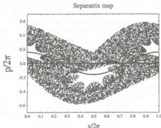
Рис. 4: The phase space portrait of separatrix map (20) for \lambda = 1 , p_0 = 0 . All points belong to a single trajectory of 10^4 iterations. The straight solid line is the usual exit line p = 0 while another one is the special exit line (23) which cuts through the two stability domains and thus blocks the contribution of their big critical structure to PR.
