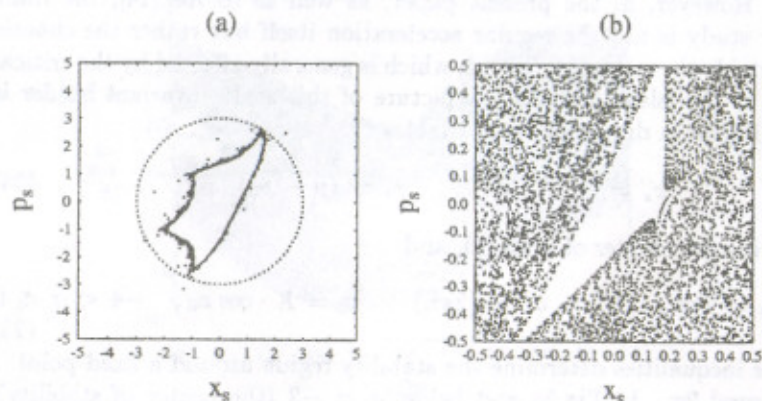
FIG. 5: Universal border of microtron islets in scaled variables (24): (a) – in the center of stability interval, \sigma = -2 , single trajectory of 5000 iterations stuck to the chaos border; (b) – near the edge of stability, \sigma \approx -3.1 , revealed by an outside trajectory of 10^7 iterations, K = 7 .
