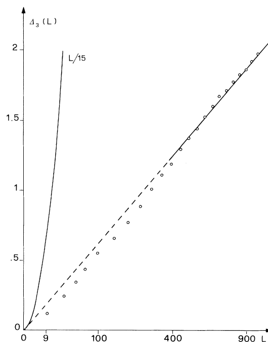
FIG. 5. Graph of ensemble average \bar{\Delta}_3(L) for L \leq 1000 showing the square-root dependence on L ; \alpha \approx 1 . The straight line fits the numerical data with \epsilon_{\text{cr}} = 0.53 .
