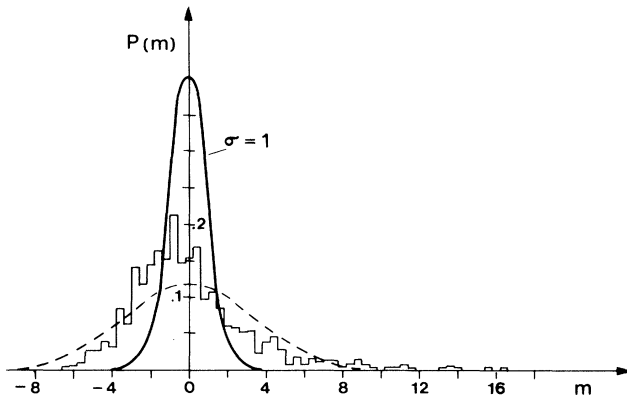
FIG. 2. Histogram of the distribution of deviations m_i = (n_i^{\text{ob}} - n^{\text{ex}}) / (n^{\text{ex}})^{1/2} of the observed number of spacings n_i^{\text{ob}} from the expected number n^{\text{ex}} in the i th interval. The intervals are so chosen that n^{\text{ex}} = 90 for each. The full line shows the Gaussian distribution of width \sigma = 1 corresponding to uncorrelated Poisson statistics; the actual observed rms width is \sigma = \sqrt{11} (dashed line).
