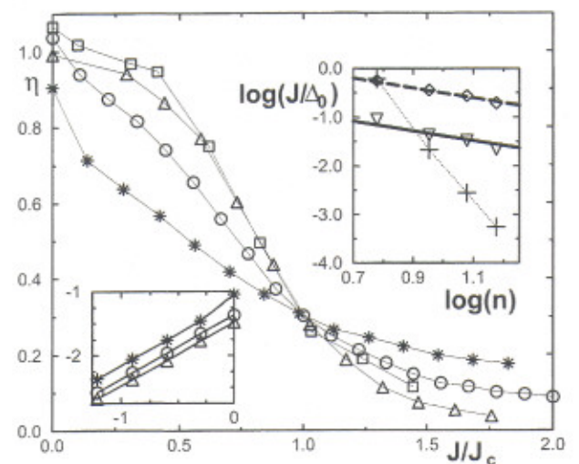
Fig. 4. Dependence of \eta on the rescaled coupling strength J/J_c for the states in the middle of the energy band for n=6 (*), 9 (o), 12 (triangles), 15 (squares); \delta = \Delta_0 . The upper insert shows \log(J_c/\Delta_0) (diamonds) and \log(J_c/\Delta_0) (triangles) versus \log(n) ; the variation of the scaled multi-qubit spacing \Delta_n/\Delta_0 with \log(n) is shown for comparison (+). Dashed line gives the theoretical formula (7) with C_q = 3.16 ; the solid line is J_c = 0.41\Delta_0/n . The lower insert shows \log(J_c/\Delta_0) versus \log(\delta/\Delta_0) for n=6 (*), 9 (o), 12 (triangles); straight lines have slope 1. After [24].
