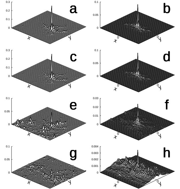
FIG. 1: Delocalization of two interacting particles with attractive Hubbard interaction U = -2V by a static electric force F . The generalized Cooper problem is considered on 2D lattice of size L \times L = 40 \times 40 at disorder strength W = 5V , a static field F is directed along y -axis. Probability is shown for a lowest energy eigenstate with a maximum probability f(y) = \sum_x f(x, y) at y = L/2 . Left panels show one-particle probability f(x, y) and right panels show interparticle distance probability f_d(x, y) . The static electric force, directed along y -axis, is F = 0 (a, b), F = 0.003V (c, d), F = 0.016V (e, f), F = 0.052V (g, h).
