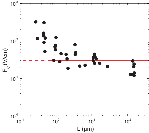
FIG. 9: (Color online) Critical field F_c for superinsulator destruction as a function of sample size L from experiments [14] (points from Fig.5 there). The theory (1) is shown by red horizontal line.
