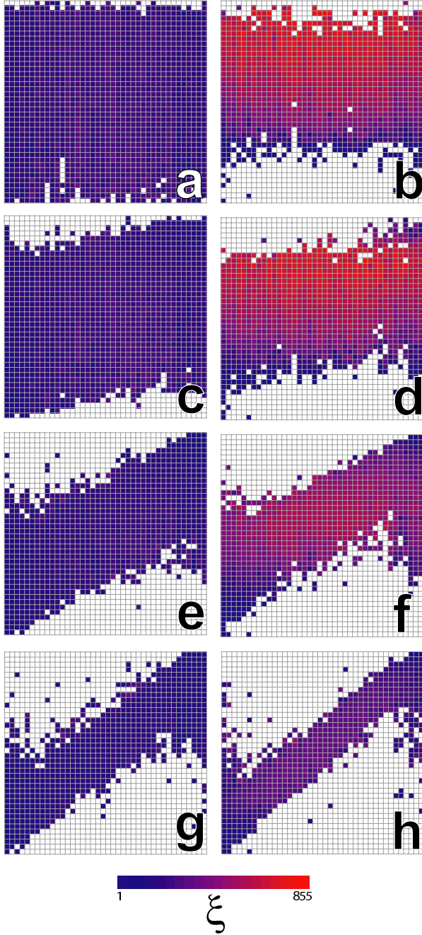
FIG. 7: (Color online) The IPR \xi for W = 5V at U = 0 (left column) and U = -2V (right column), at different values of the static force F = 0 (a,b), F = 0.004V (c,d), F = 0.016V (e,f), F = 0.04V (g,h). Each panel has 40 \times 40 cells, the vertical direction corresponds to the coupling energy \Delta E = E - 2E_F , the horizontal one to 1 \leq y \leq 40 . The bottom row corresponds to the lowest coupling energy, and the upper row corresponds to the highest coupling energy within the energy intervals at U = 0 being (0, 0.54V) (a), (-0.05V, 0.59V) (c), (-0.25V, 0.78V) (e), (-0.69V, 1.18V) (g) and at U = -2V being (-0.2V, 0.39V) (b), (-0.23V, 0.57V) (d), (-0.39V, 0.75V) (f), (-0.77V, 1.17V) (h). The cell color gives the average \xi inside the cell (with \Delta E being in the corresponding energy range defined by the row, and the maximum of probability distribution f(y) along y , being located at y position defined by the column). For each panel \sim 30000 states are used with N_d = 30 disorder realizations. These states are selected in such a way that the probability of two particles located at the same site is greater than 5/L(2L - 1) ; here L = 40 .
