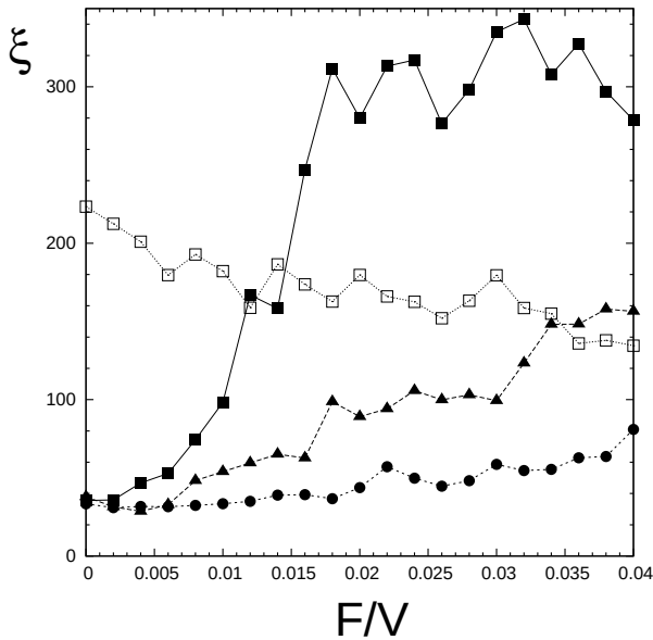
FIG. 4: Dependence of the average IPR \xi of lowest energy states on the static force F ; average is done over N_l = 15 lowest energy states with a maximum of f(x, y) inside a stripe 0.4L \leq y \leq 0.6L in a middle of the lattice at y = L/2 for N_D = 30 disorder realizations; the lattice size is L = 20 ( \bullet ), L = 30 ( \blacktriangle ), L = 40 ( \blacksquare ) at U = -2V ; the values of \xi for noninteracting case are shown by open symbols ( \square ) for L = 40, U = 0 . Here W = 5V .
