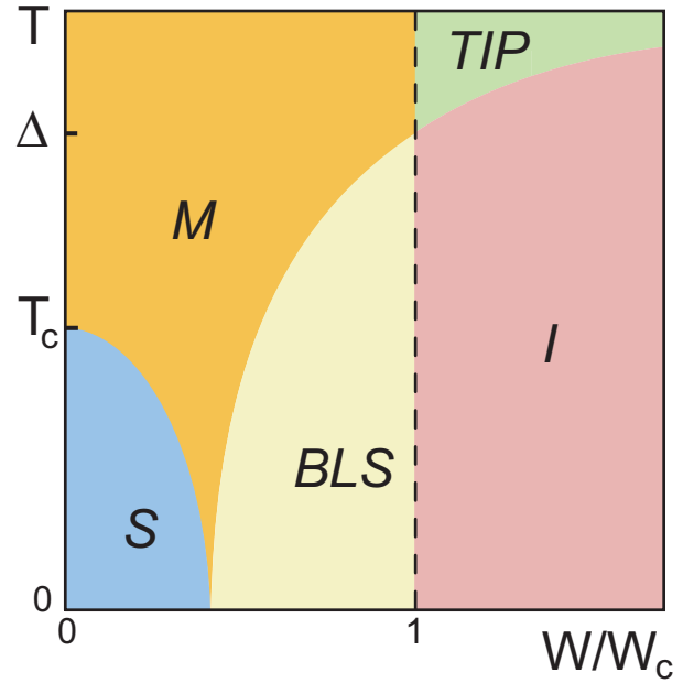
FIG. 10: (Color online) Schematic phase diagram in the temperature-disorder plane (T, W) for quasi-2D or 3D Anderson model at fixed Hubbard attraction U = -2V and fixed filling factor with the Fermi energy E_F : the vertical dashed line shows the Anderson transition at W = W_c \approx 16.5V for noninteracting particles, S is the superconducting phase, BLS is the insulator phase of localized BLS pairs, M is essentially the noninteracting metallic phase, TIP is the metallic phase of delocalized TIP pairs. Here we assume T \ll E_F , static field is zero, temperature linear axis is shown in arbitrary units.
