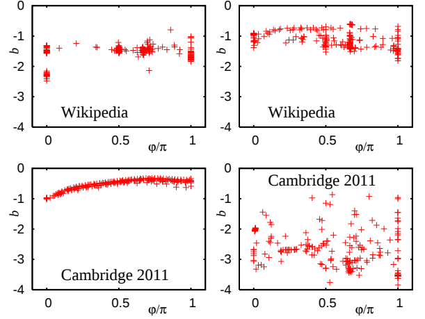
Fig. 4. Left column: Algebraic exponent b obtained from a power law fit |\psi_i(K_i)| \sim K_i^b for K_i \geq 10^4 shown as a function of the phase \varphi = \arg(\lambda_i) of the complex eigenvalue \lambda_i associated to the eigenvector \psi_i of S . The shown data points correspond to the eigenvalue selection of Fig. 3 for networks of Wikipedia and Cambridge 2011. Right column: The same as in the left column for the eigenvectors of S^* .
