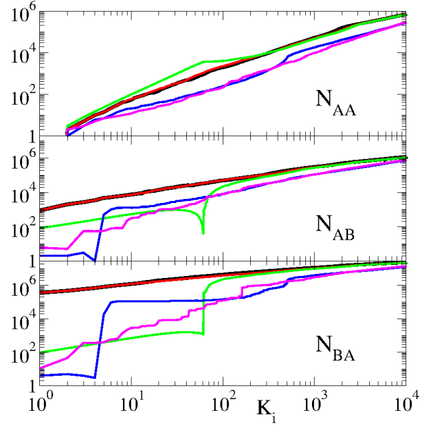
Fig. 9. Number of links between or inside sets A and B defined by the index K_i ordered by decreasing absolute value of Wikipedia eigenstates. The number of links starting and pointing to nodes inside the set A ( N_{AA} ) is shown in top panel as a function of K_i . The cases of links from set A to set B ( N_{AB} ) and from B to A ( N_{BA} ) are shown in middle and bottom panel respectively. Note that the total number of links is conserved and the quantity N_{BB} can be obtained as N_{BB} = N_\ell - N_{AA} - N_{AB} - N_{BA} . The case of PageRank vector with damping parameter \alpha = 0.85 is shown by a black curve versus K index. The color curves show the cases of four core space eigenvectors |\psi_i\rangle of S versus their ranking indexes K_i . Red and green curves are the eigenvectors corresponding to the two largest core space eigenvalues (in modulus) being \lambda_1 = 0.99998702 and \lambda_2 = 0.97723699 respectively; blue and pink curves are the eigenvectors corresponding to two complex eigenvalues with large imaginary part being \lambda_{52} = -0.35003316 + i0.77373677 and \lambda_{864} = -0.34293502 + i0.43144930 respectively.
