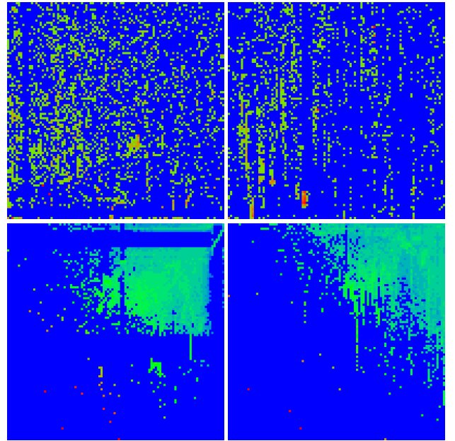
Fig. 8. Density of nodes W(K, K^*) on PageRank-CheiRank plane (K, K^*) for the networks of BBC (left panels) and Le Monde (right panels). Top panels show density in the range 1 \leq K, K^* \leq 10^4 with averaging over cells of size 100 \times 100 ; bottom panels show density averaged over 100 \times 100 logarithmically equidistant grids for 0 \leq \ln K, \ln K^* \leq \ln N , the density is averaged over all nodes inside each cell of the grid, the normalization condition is \sum_{K, K^*} W(K, K^*) = 1 . Color varies from blue at zero value to red at maximal density value. At each panel the x -axis corresponds to K (or \ln K for the bottom panels) and the y -axis to K^* (or \ln K^* for the bottom panels).
