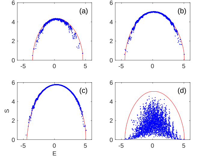
Fig. 4: (Color on-line) Dependence of entropy on energy S(E) for (a) M = 12 , L = 5 , N = 792 , J = 1 ; (b) M = 16 , L = 7 , N = 3003 , J = 1 ; (c) M = 14 , L = 6 , N = 11440 , J = 1 ; (d) M = 16 , L = 7 , N = 3003 , J = 0.1 . Blue points show the numerical data E_m, S_m for all eigenstates, the red curves show the theoretical Fermi-Dirac thermal distribution (3). Here V = \sqrt{14} .
