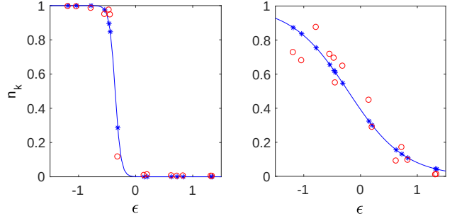
Fig. 2: (Color on-line) Dependence of filling factors n_k on energy \epsilon for individual eigenstates obtained from exact diagonalization of (2) (red circles) and from the Fermi-Dirac ansatz with one-particle energy \epsilon (3) (full blue curve; blue stars are shown at one-particle energy positions \epsilon = \epsilon_k ). Here M = 14, L = 6, N = 3003, J = 1, V = \sqrt{14} and eigenenergies (2) are E = -4.4160 (left panel), -3.0744 (right panel); the theory blue curves (3) are drawn for the temperatures corresponding to these energies \beta = 1/T = 20 (left panel), 2 (right panel), see Fig. 3(b) below.
